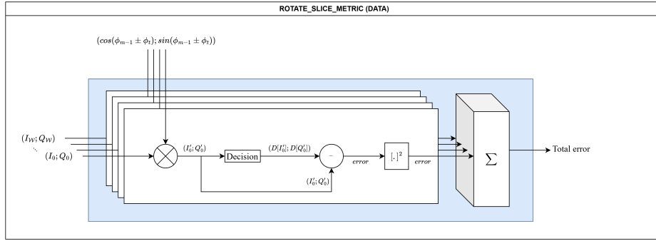
Figure 4.8: Datapath diagram of the rotate metric slice unit
