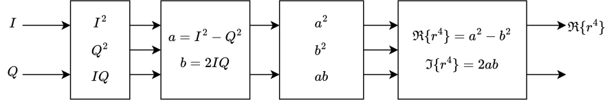
Figure 4.15: Calculation-flow of the fourth-power module
