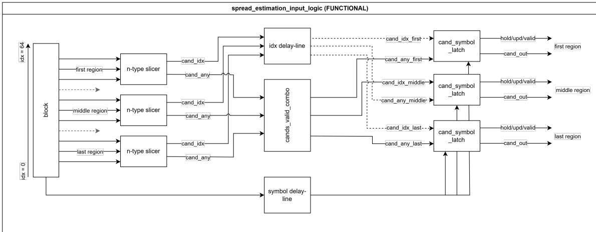
Figure 4.13: Functional diagram of the SE input selector
