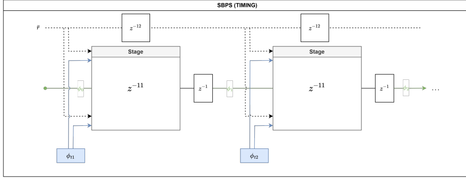
Figure 4.9: Timing diagram of the full SBPS algorithm
