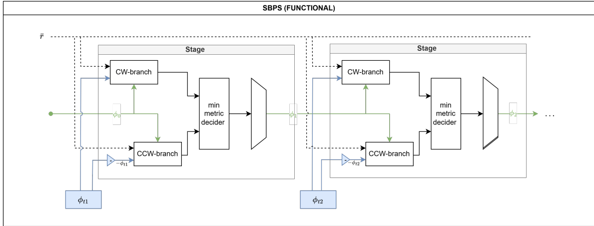
Figure 4.3: Functional diagram of the full SBPS architecture
