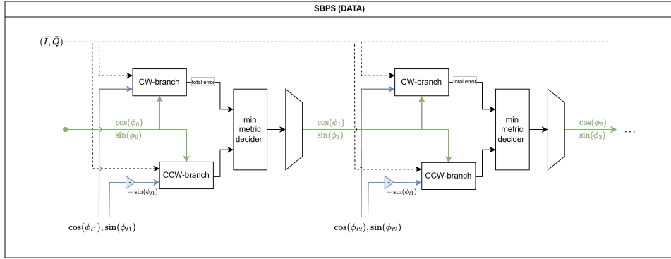
Figure 4.6: Datapath diagram of the full SBPS architecture
