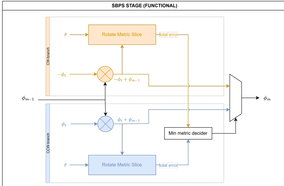
Figure 4.4: Functional diagram of the SBPS stage
