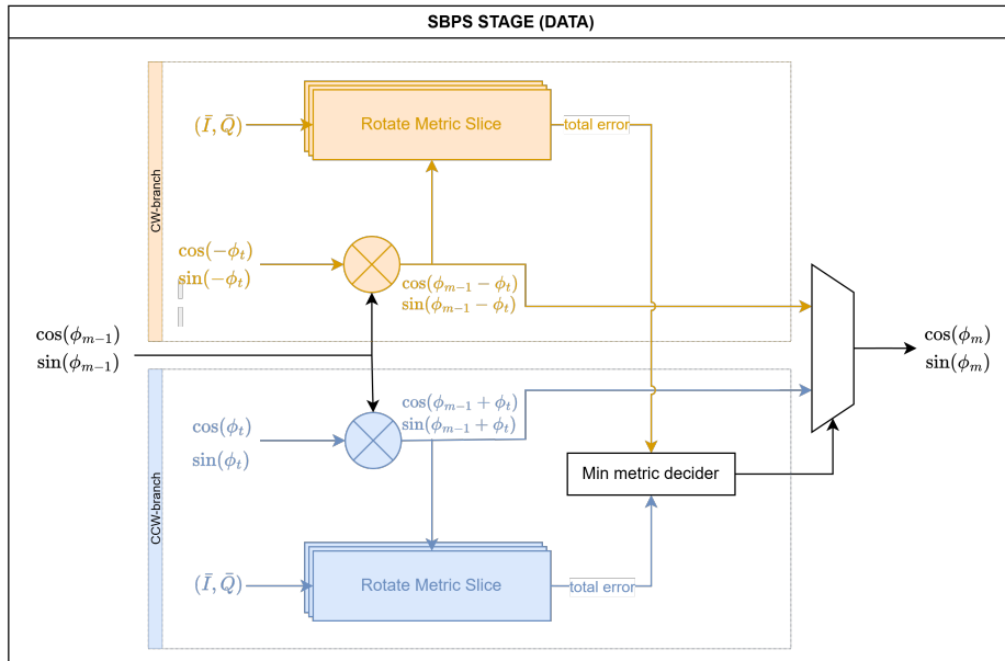
Figure 4.7: Datapath diagram of the SBPS stage
