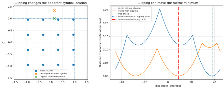
Figure 4.1: Clipping causing false minima for SBPS metric
