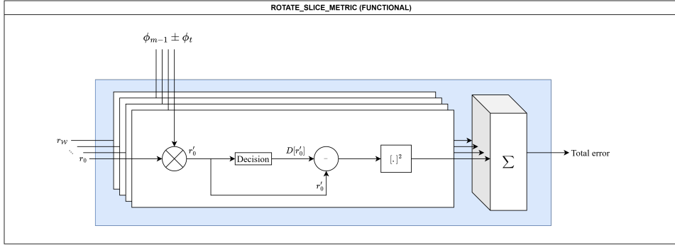
Figure 4.5: Functional diagram of the rotate metric slice unit
