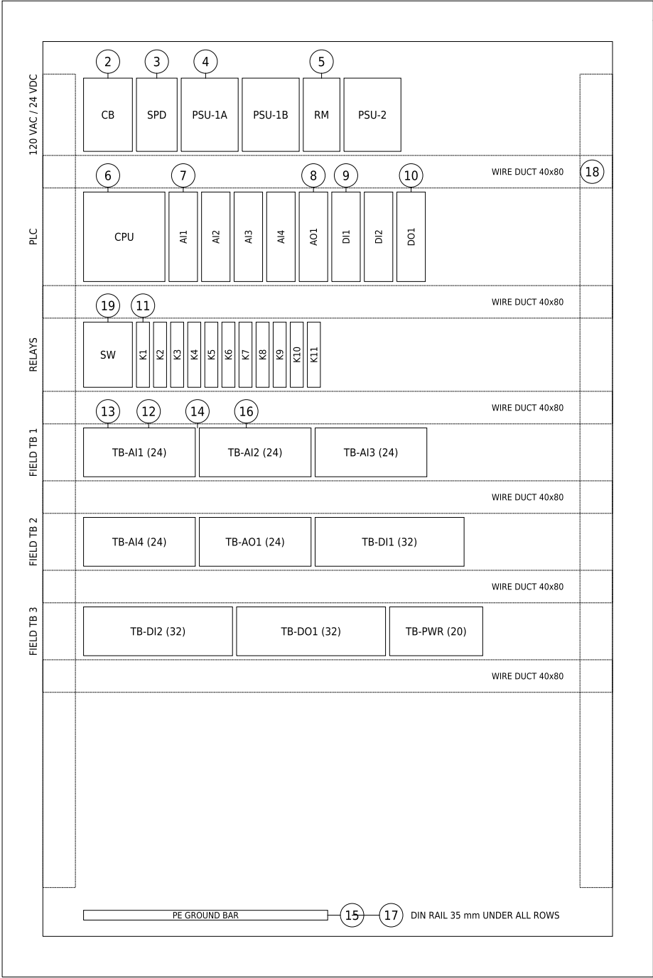
BACKPLATE VIEW SCALE 1:6 ENCLOSURE 1200 H x 800 W x 300 D, BACKPLATE 1100 x 700
