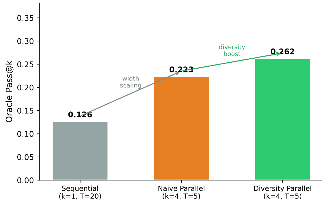
(a) Oracle Accuracy
