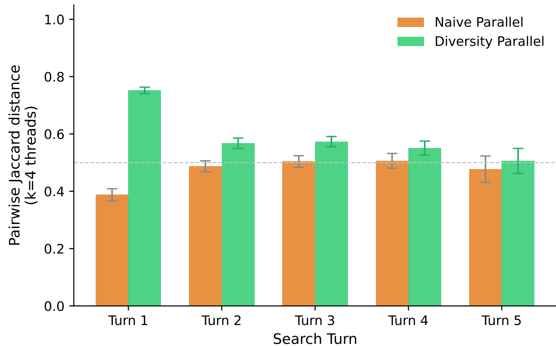
(b) Anchor Collapse — Query Diversity per Turn
