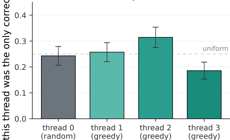
Single-correct thread | qwen3-4b x musique (n = 140 questions)
