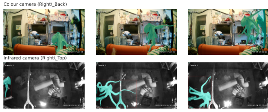
Fig. 3. Auto-labelling teacher (GroundingDINO+SAM2) masks tracked across a clip on a colour camera (top) and an infrared camera (bottom). SAM2 video propagation with largest-blob and area-continuity cleanup yields the temporally consistent masks used to train the student.
