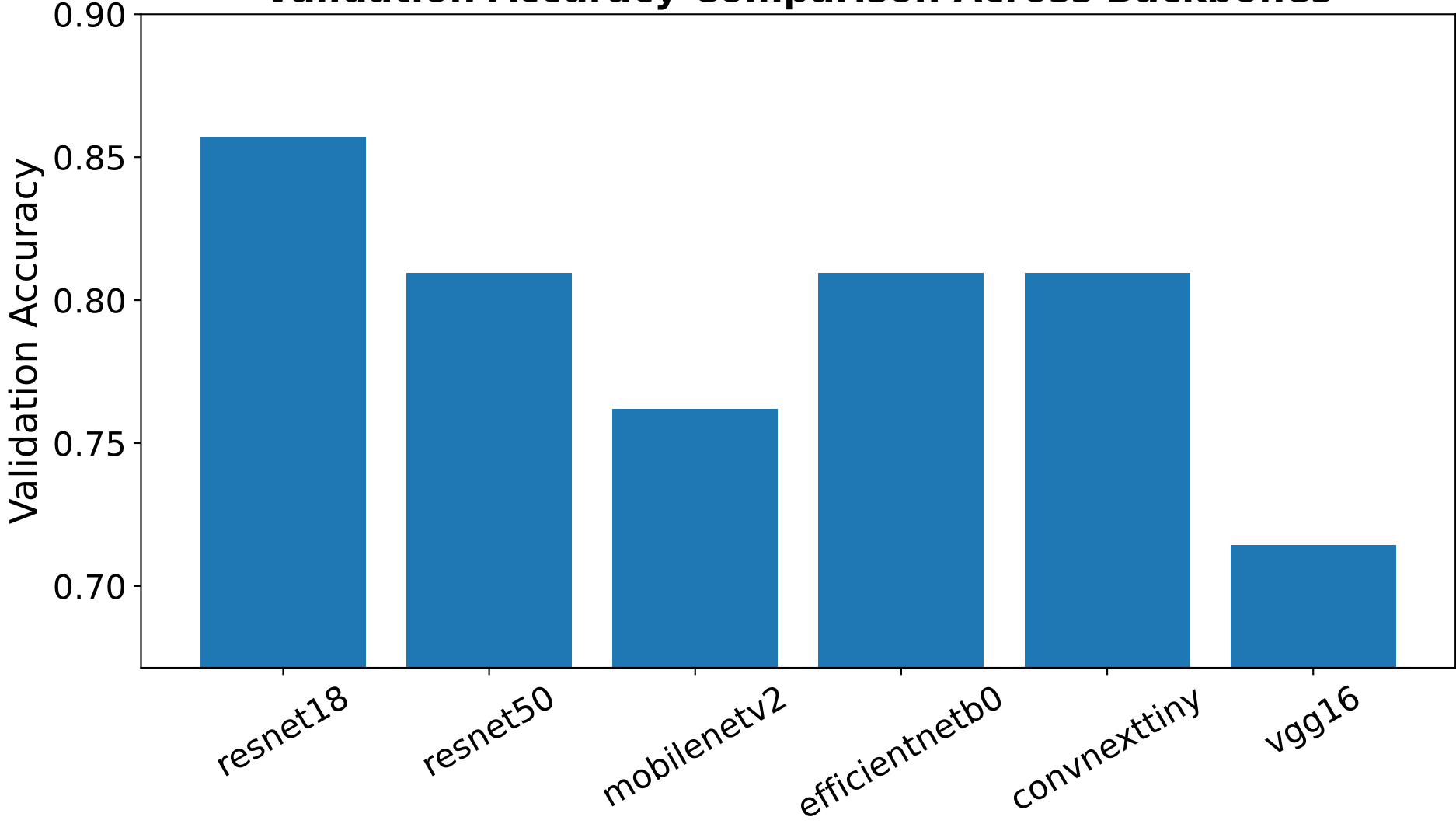
Validation Accuracy Comparison Across Backbones
