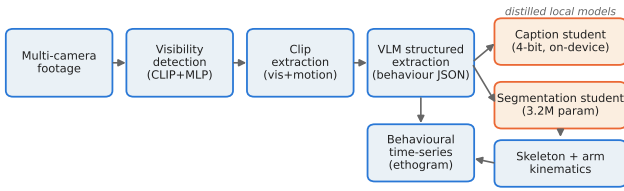
Fig. 1. Footage-to-ethogram pipeline (the four stages of Sec. III): visibility detection \rightarrow clip extraction \rightarrow VLM structured behavioural extraction \rightarrow distillation into local caption and segmentation students.
