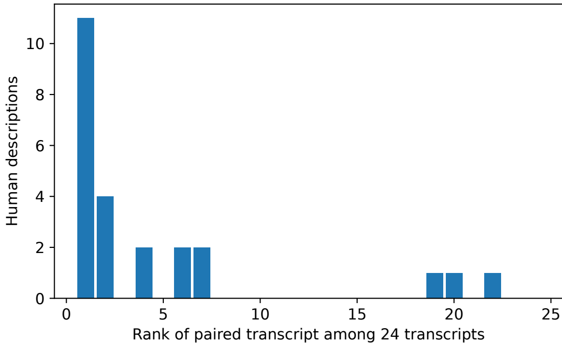
Transcript retrieval (exploratory input-text diagnostic)
