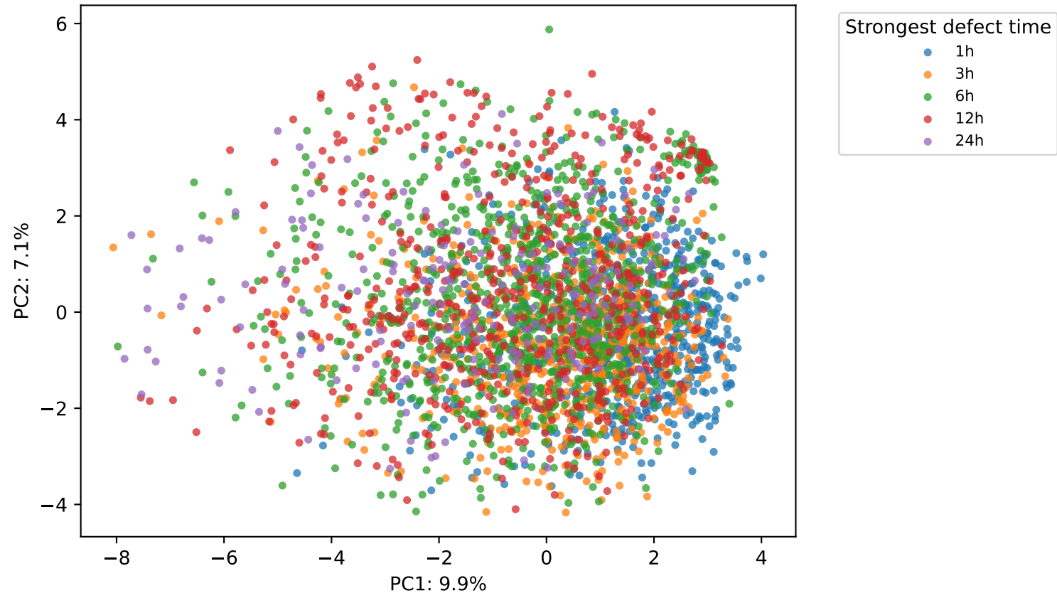
PCA of 5 × 12 spatiotemporal fitness profiles Each point is one gene; color = time of strongest fitness defect
