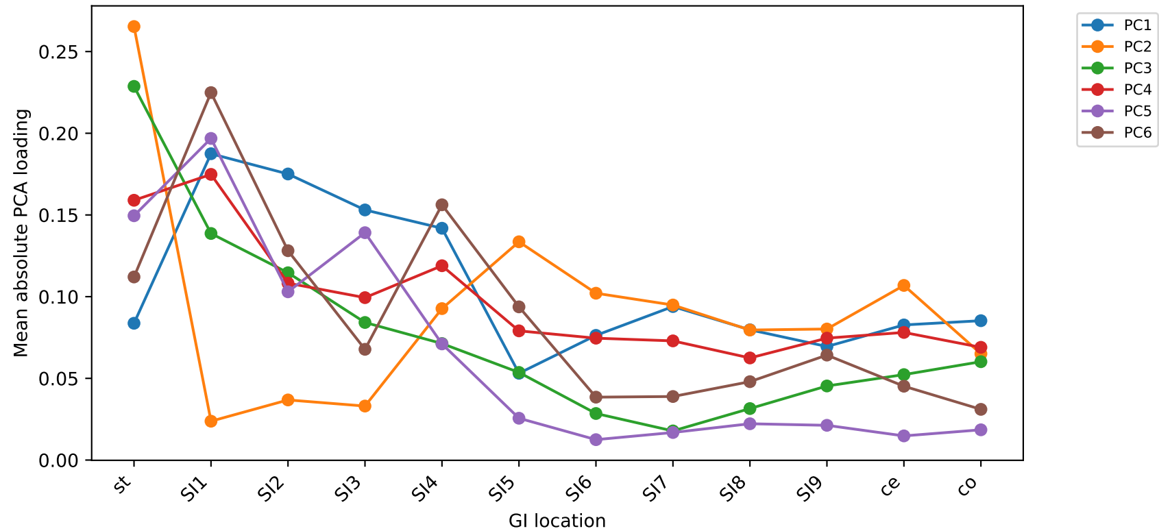
Spatial strength of PCA linear programs
