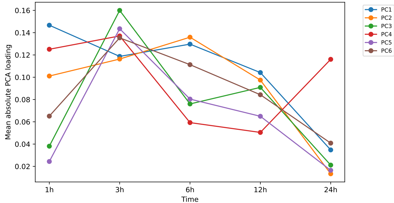
Temporal strength of PCA linear programs
