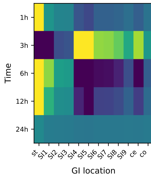
TensorComp5
