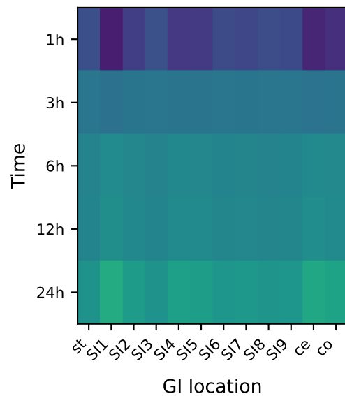
TensorComp4
