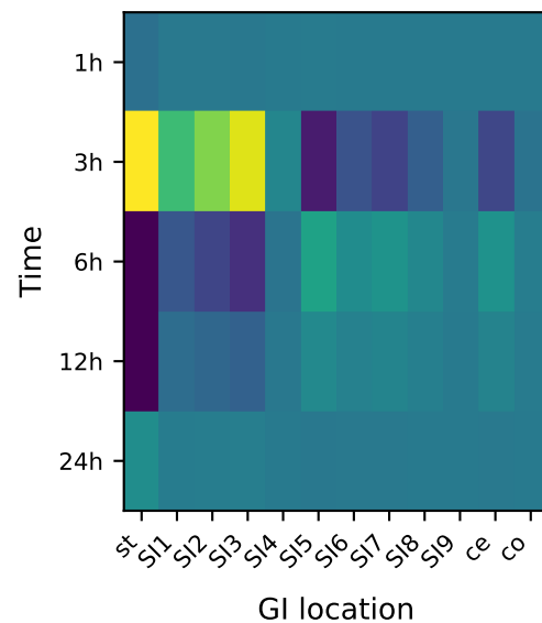
TensorComp3
