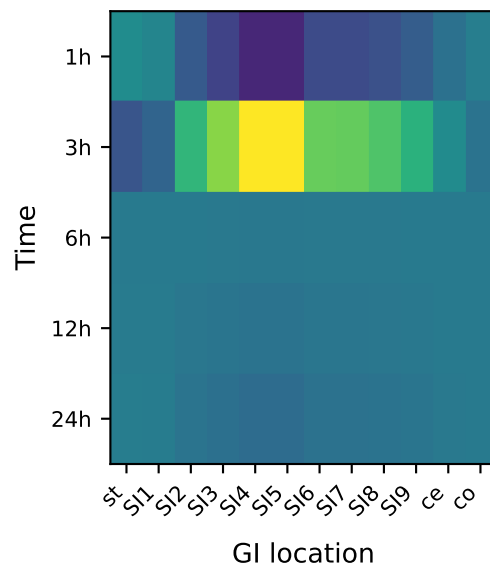
TensorComp2
