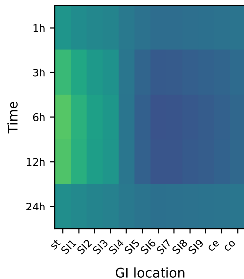
TensorComp1
