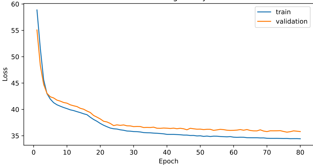
VAE training history
