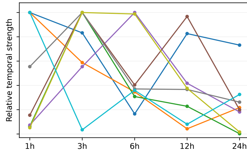
weighted CPVAE
