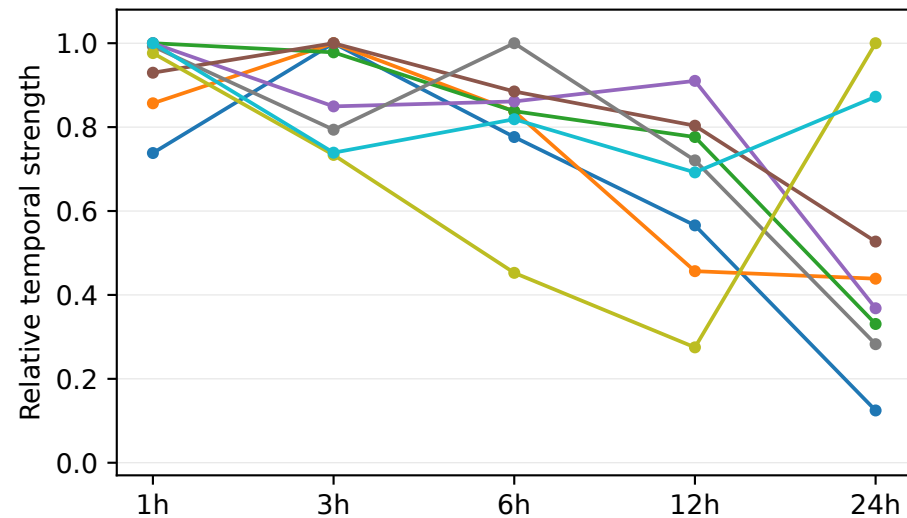
VAE
