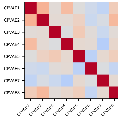
weighted CPVAE
