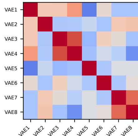
VAE
