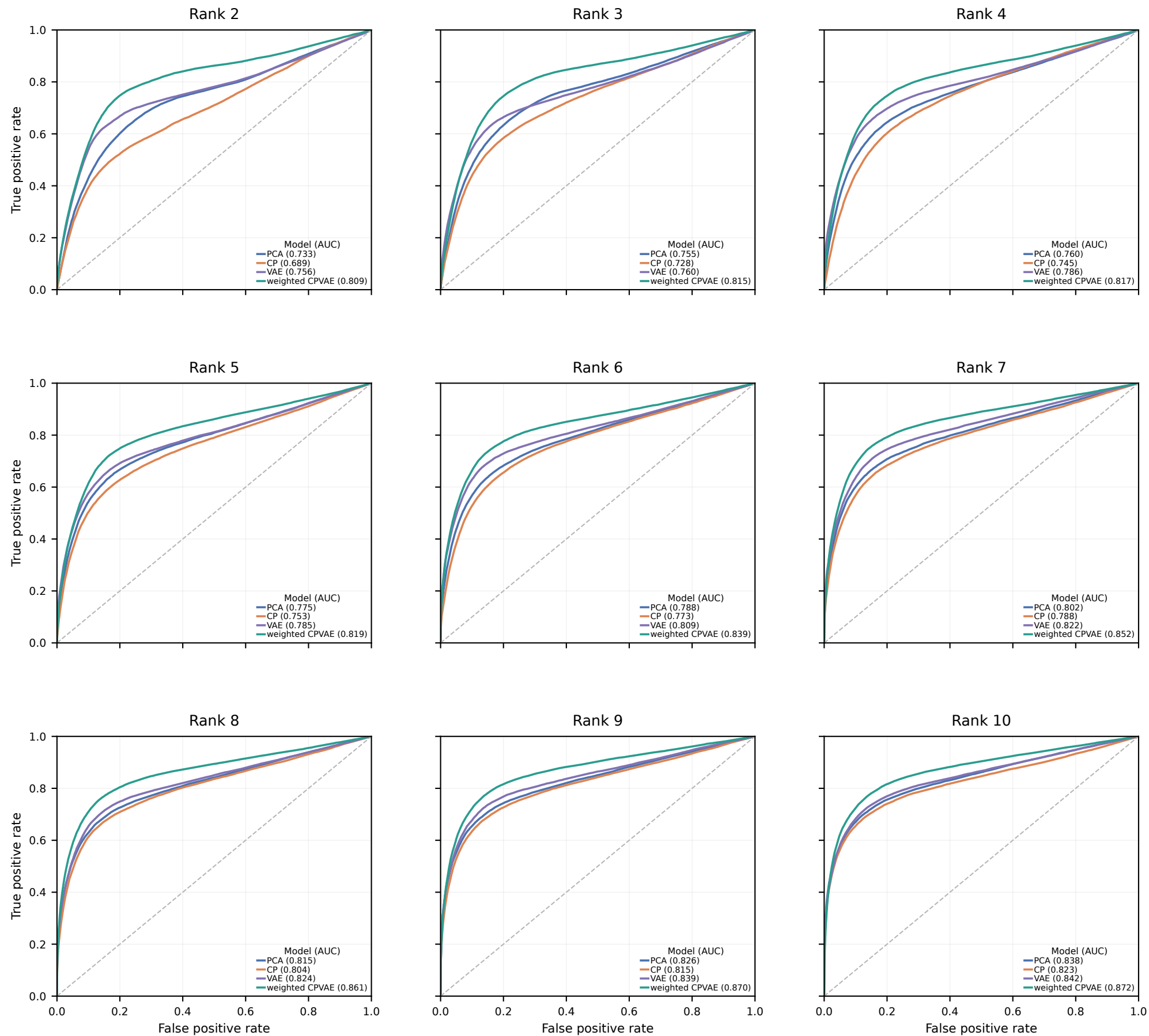
Rank2-rank10 reconstruction ROC curves across four models
