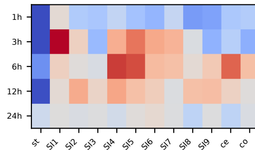
VAE 1
