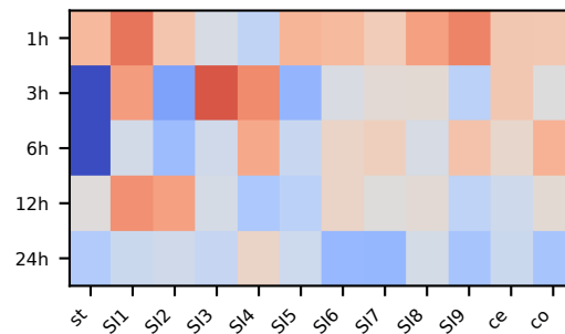
VAE 2
