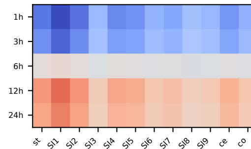
weighted CPVAE 1
