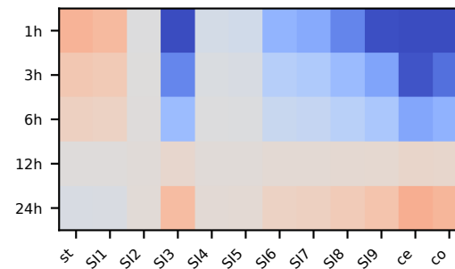
weighted CPVAE 2
