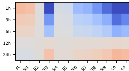
weighted CPVAE 2
