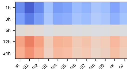
weighted CPVAE 1
