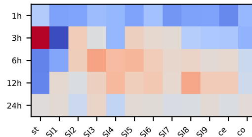
VAE 3
