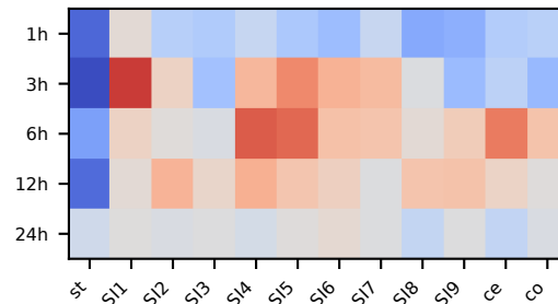
VAE 1
