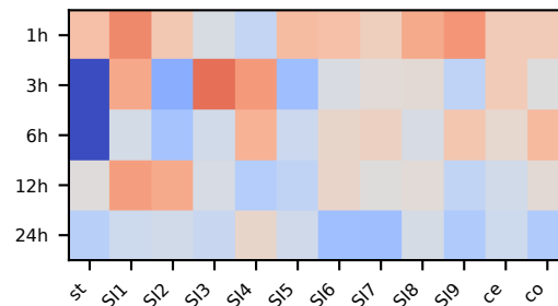
VAE 2
