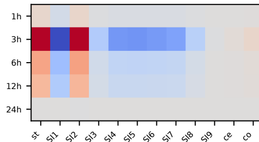
weighted CPVAE 3
