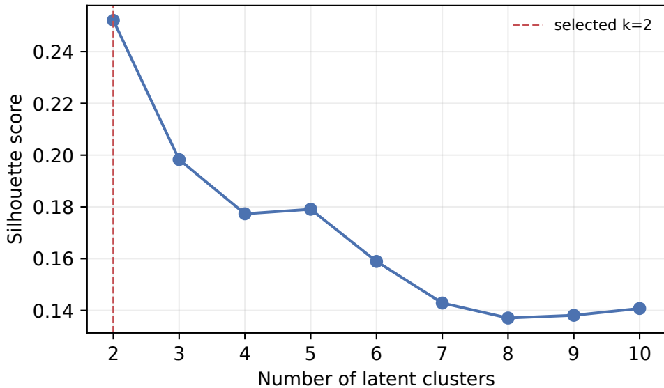
CPVAE latent cluster selection
