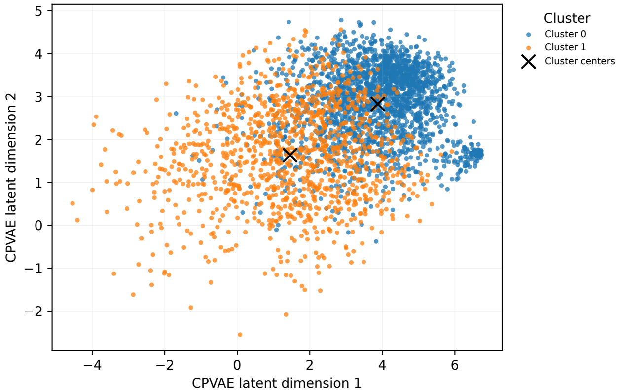
CPVAE rank8 latent clusters / nonlinear programs
