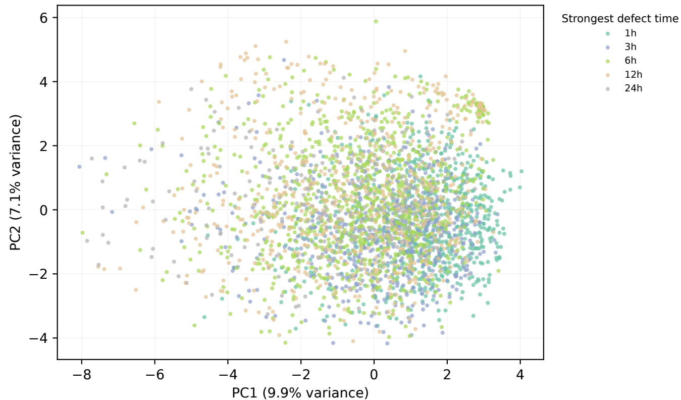
PCA gene map colored by strongest defect time
