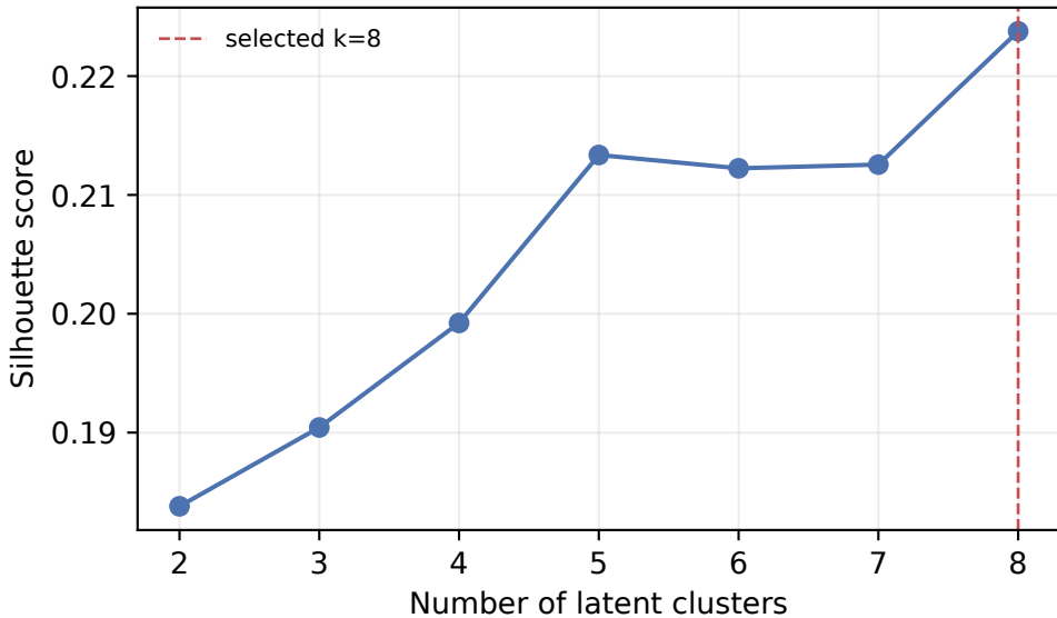
VAE latent cluster selection
