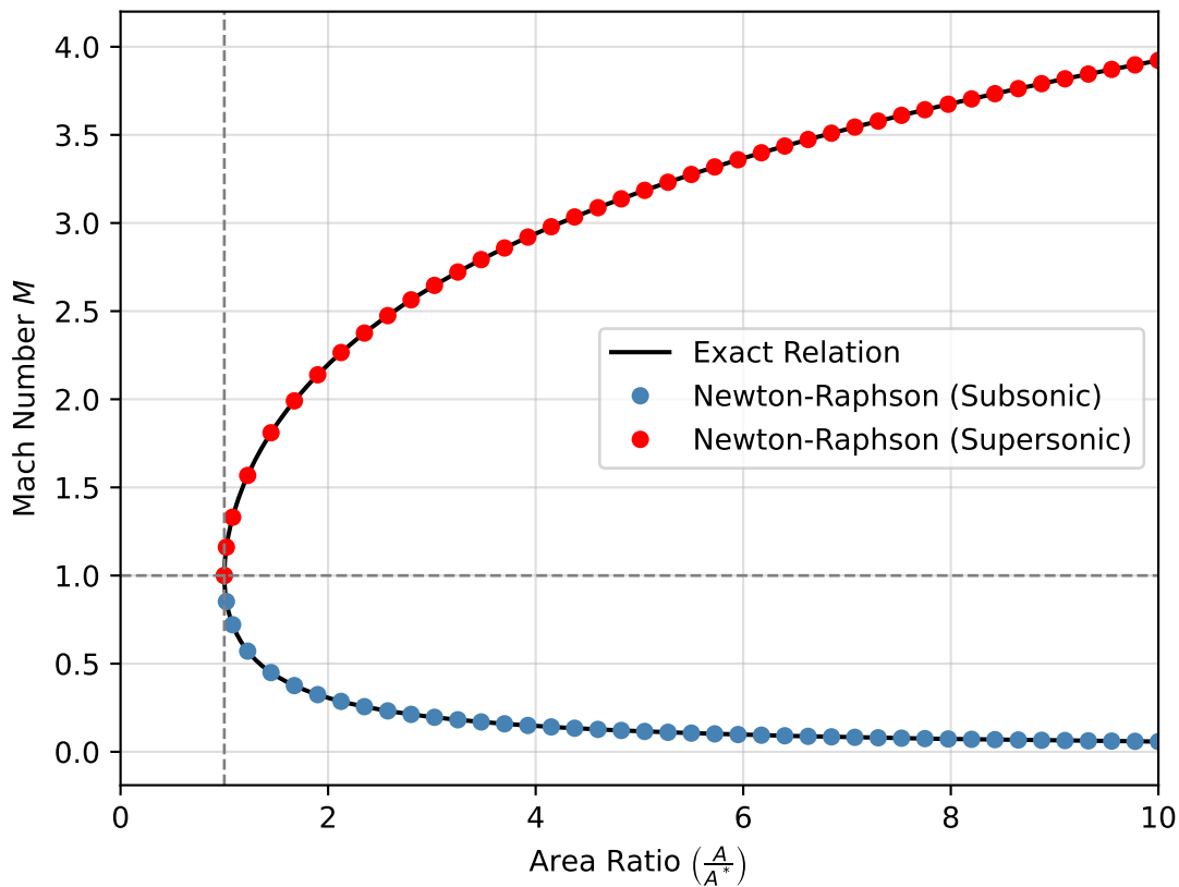
Nozzle Area-Mach Relation ( \gamma = 1.4 )
