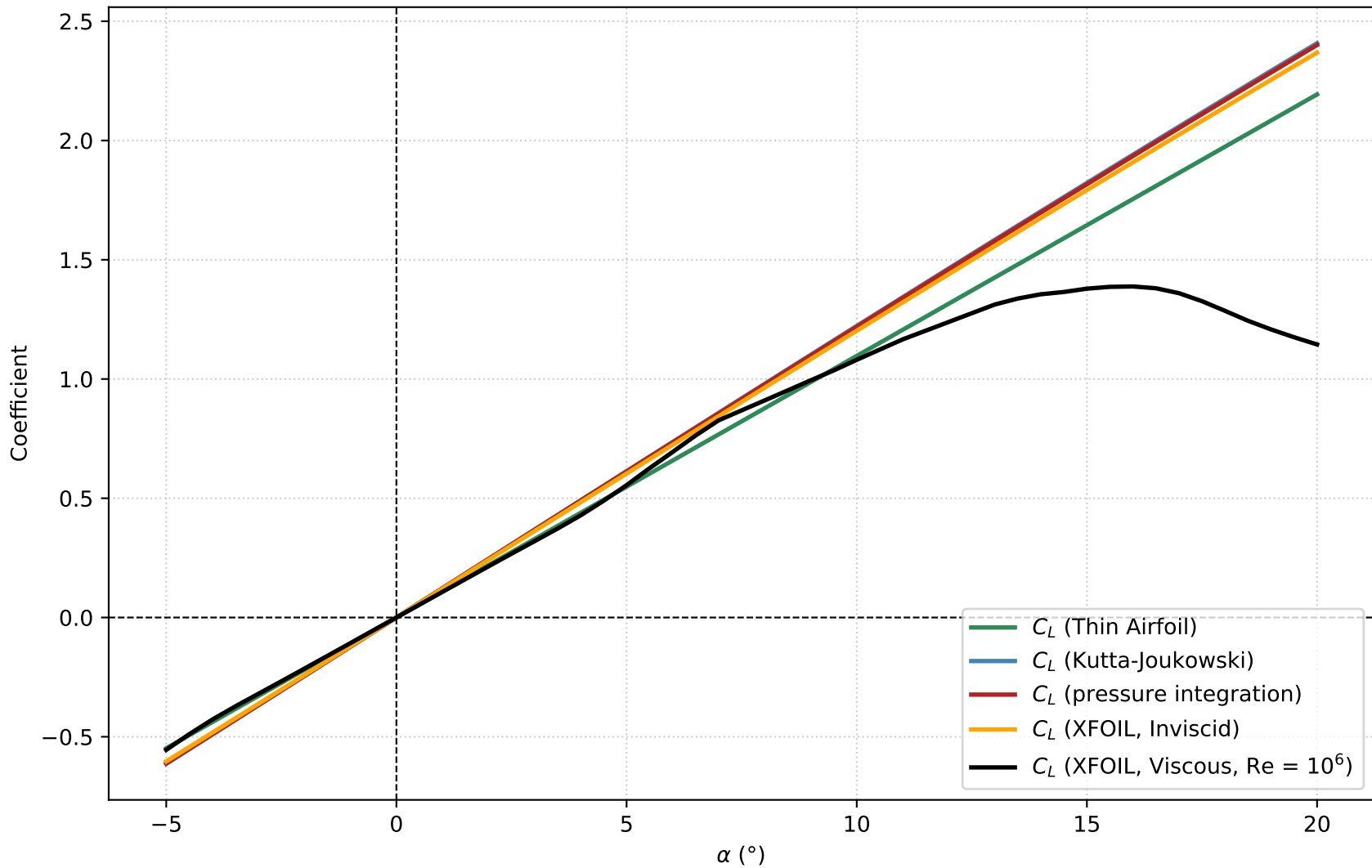
C_L vs. \alpha (NACA 0012, 199 panels)
