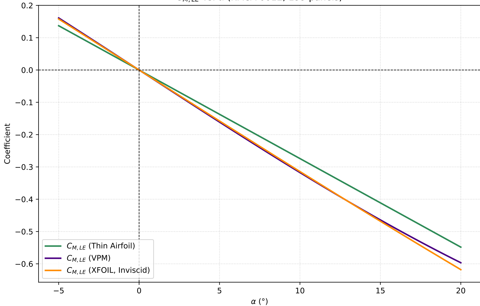
C_{M,LE} vs. \alpha (NACA 0012, 199 panels)
