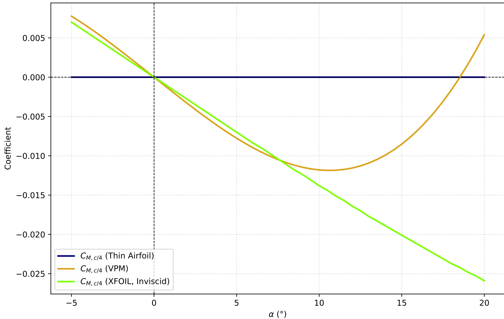
C_{M, c/4} vs. \alpha (NACA 0012, 199 panels)
