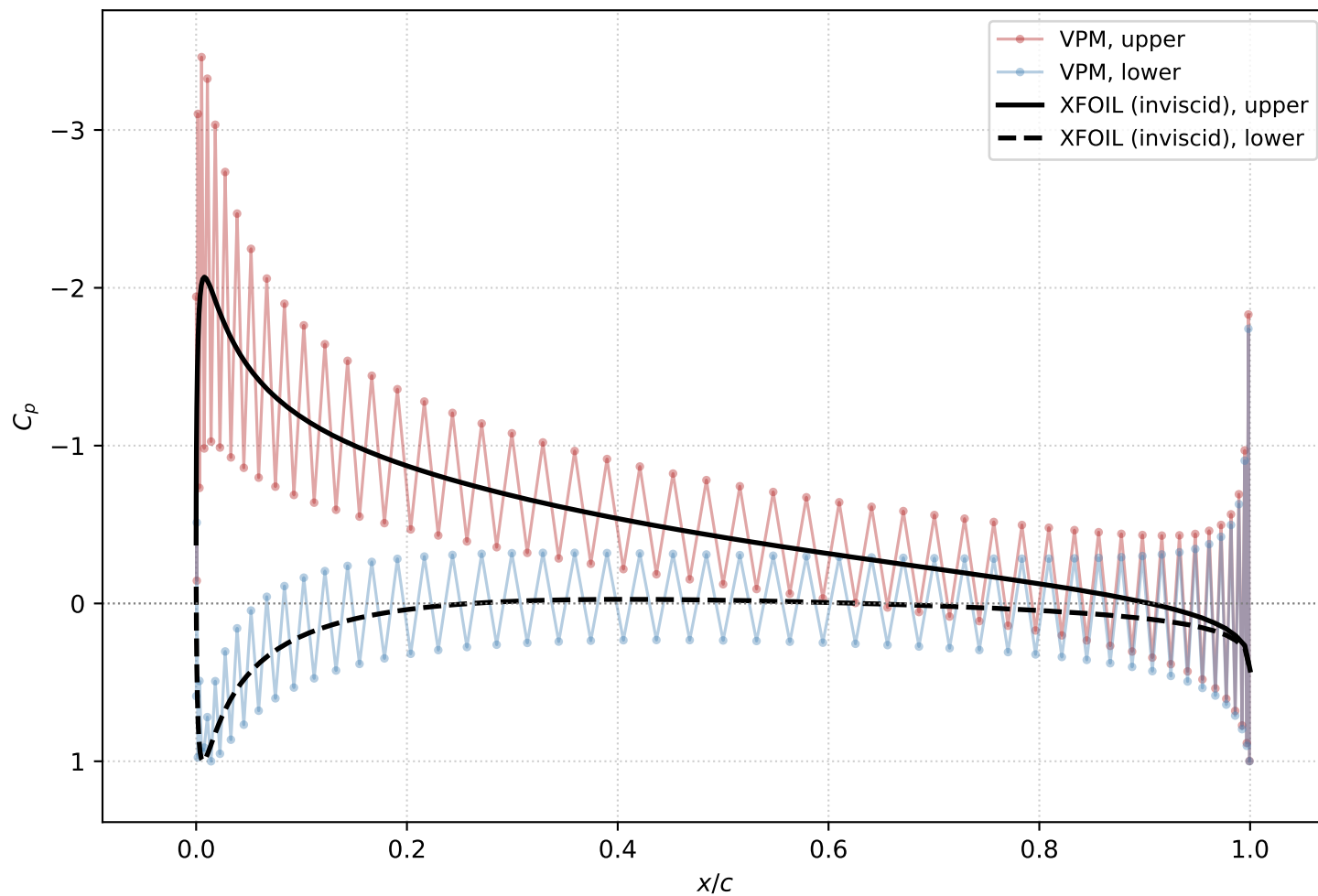
C_p VPM vs. XFOIL Inviscid (NACA 0012, \alpha = 5.0^\circ , 199 panels)
