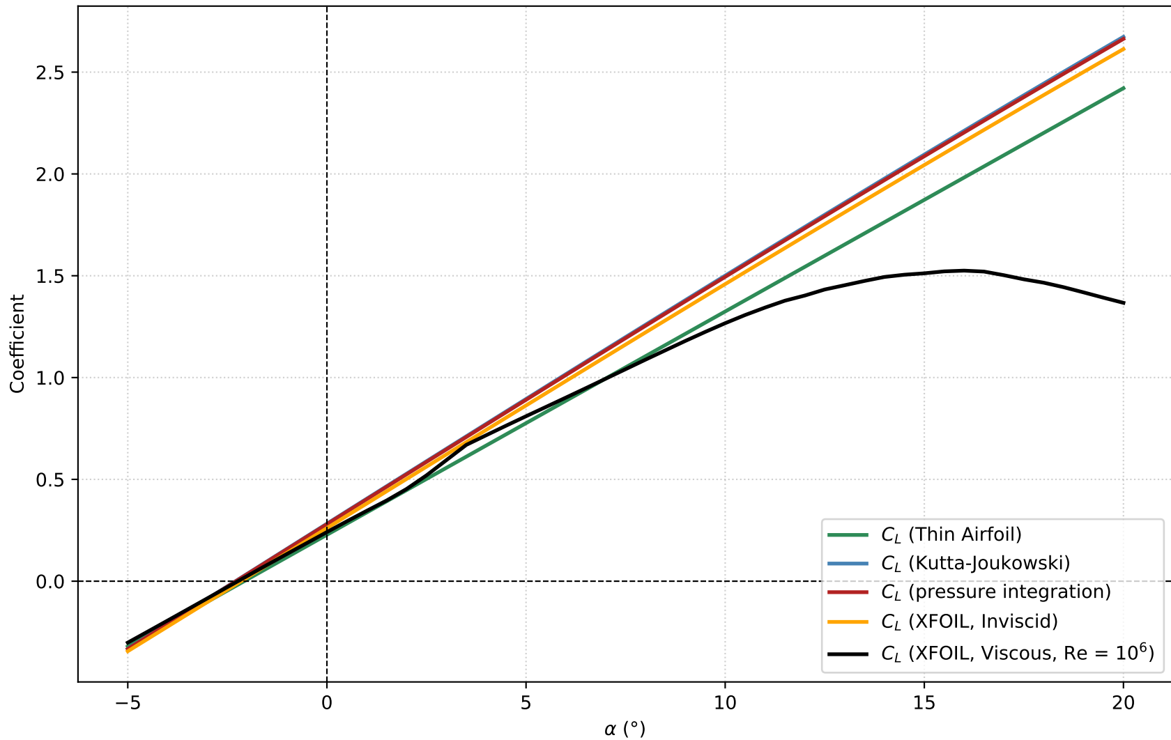
C_L vs. \alpha (NACA 2412, 199 panels)
