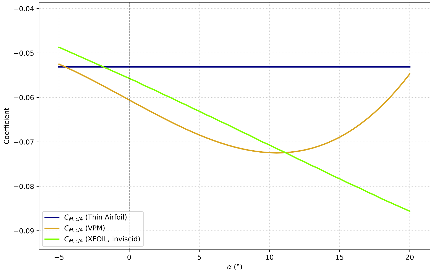
C_{M,c/4} vs. \alpha (NACA 2412, 199 panels)
