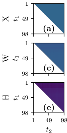
Rxn1 2% noise
