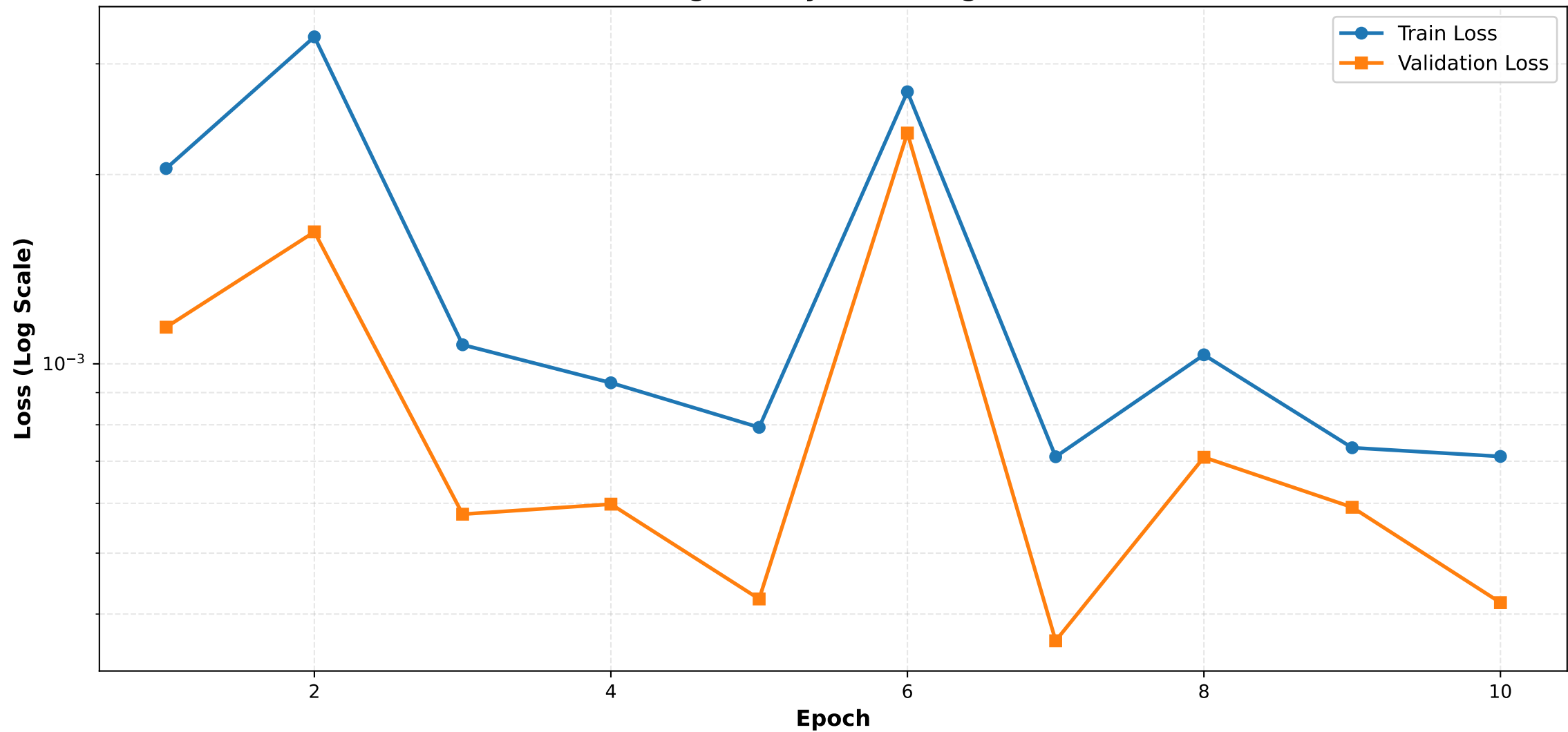
Training History: Loss (Log Scale)
