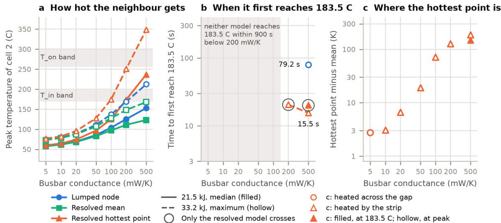
Figure 1. Registered runs, two strips, 30 s release. (a) Peak temperatures against the two-sigma bands of T_{in} and T_{on} and (b) first time each model reaches 183.5 C, at the median (filled) and maximum (hollow) energy. (c) Hottest point minus mean at the median energy, at its peak (hollow) and on reaching 183.5 C (filled); triangles are heated mainly by a strip, circles across the gap.
