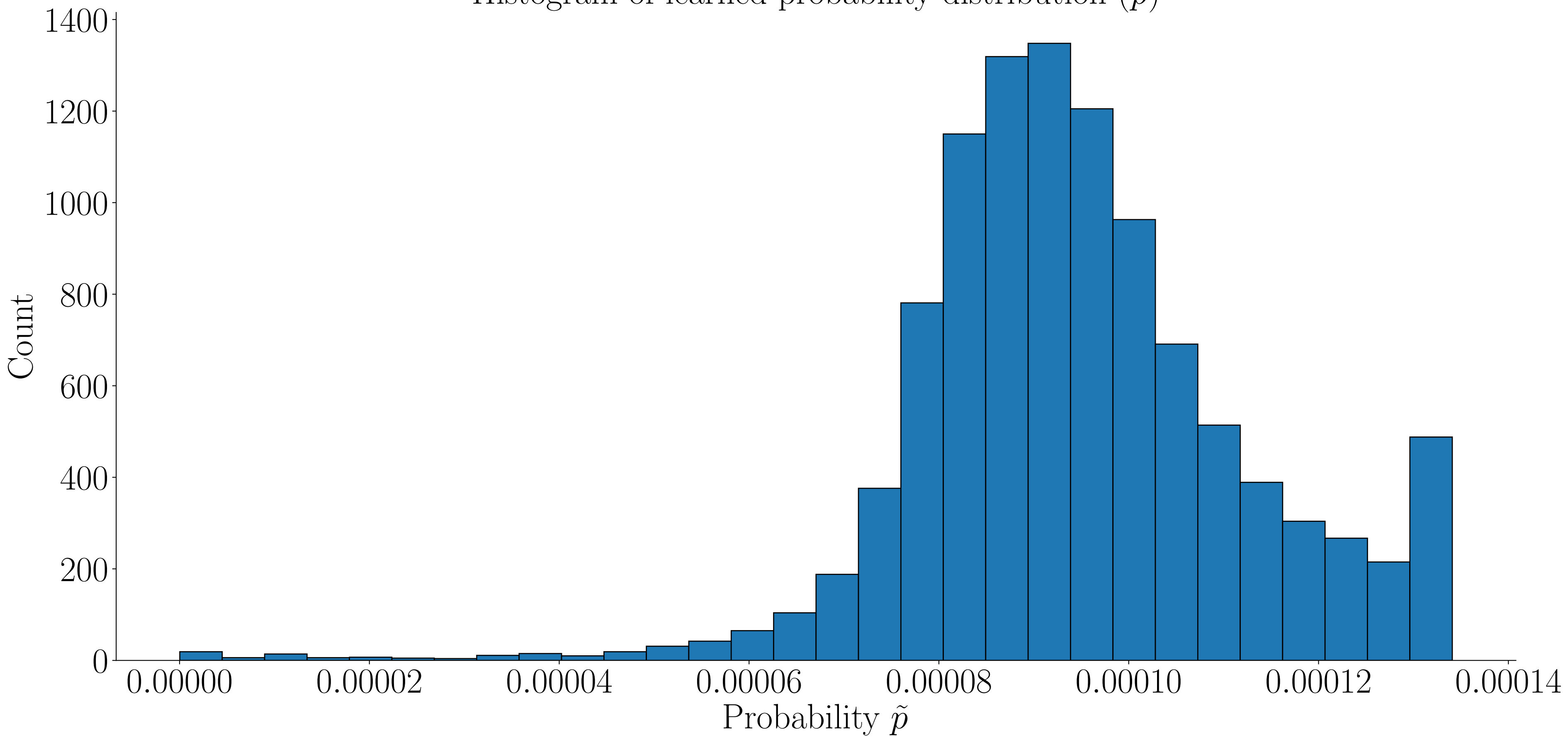
Histogram of learned probability distribution ( \tilde{p} )
