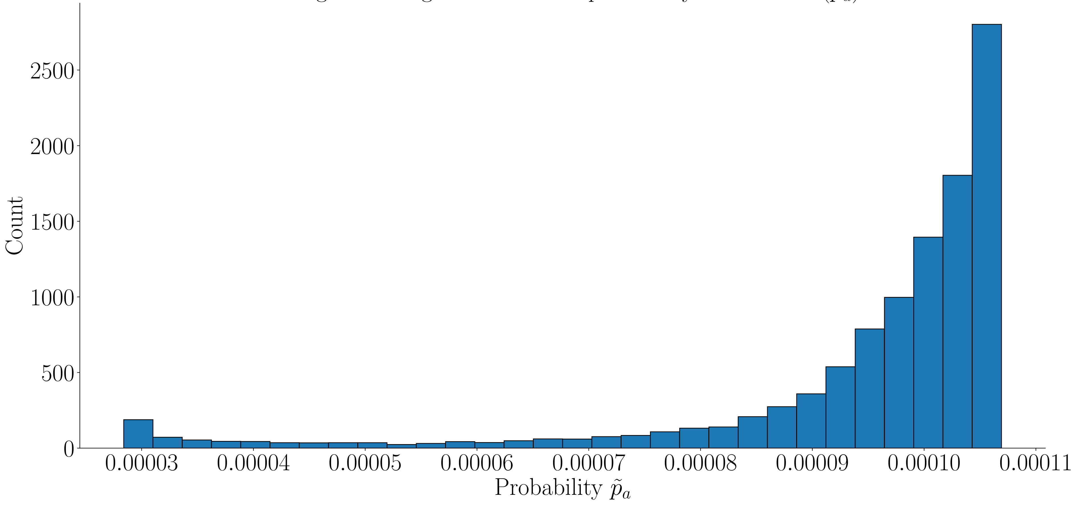
Histogram of augmented learned probability distribution ( \tilde{p}_a )
