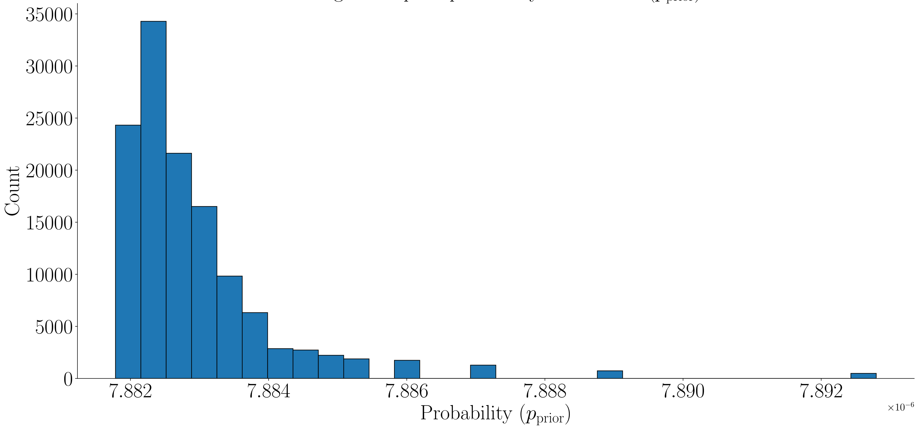
Histogram of prior probability distribution ( p_{\text{prior}} )
