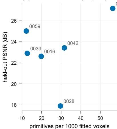
(a) the naive reading: quality vs budget
