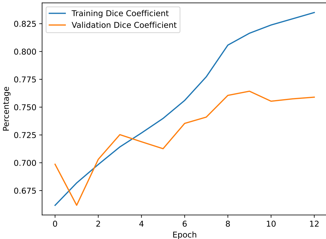
Attention U-NET for Retinal Vessel Segmentation: Dice Coefficient Metric
