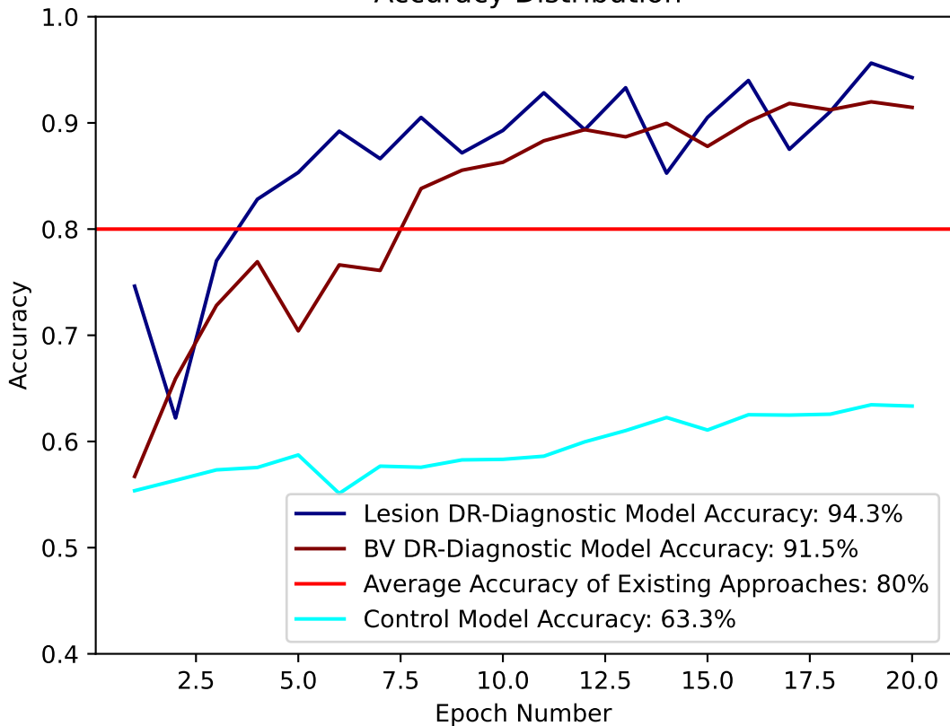
Inception-v3 DR-Diagnostic and Control Models: Accuracy Distribution
