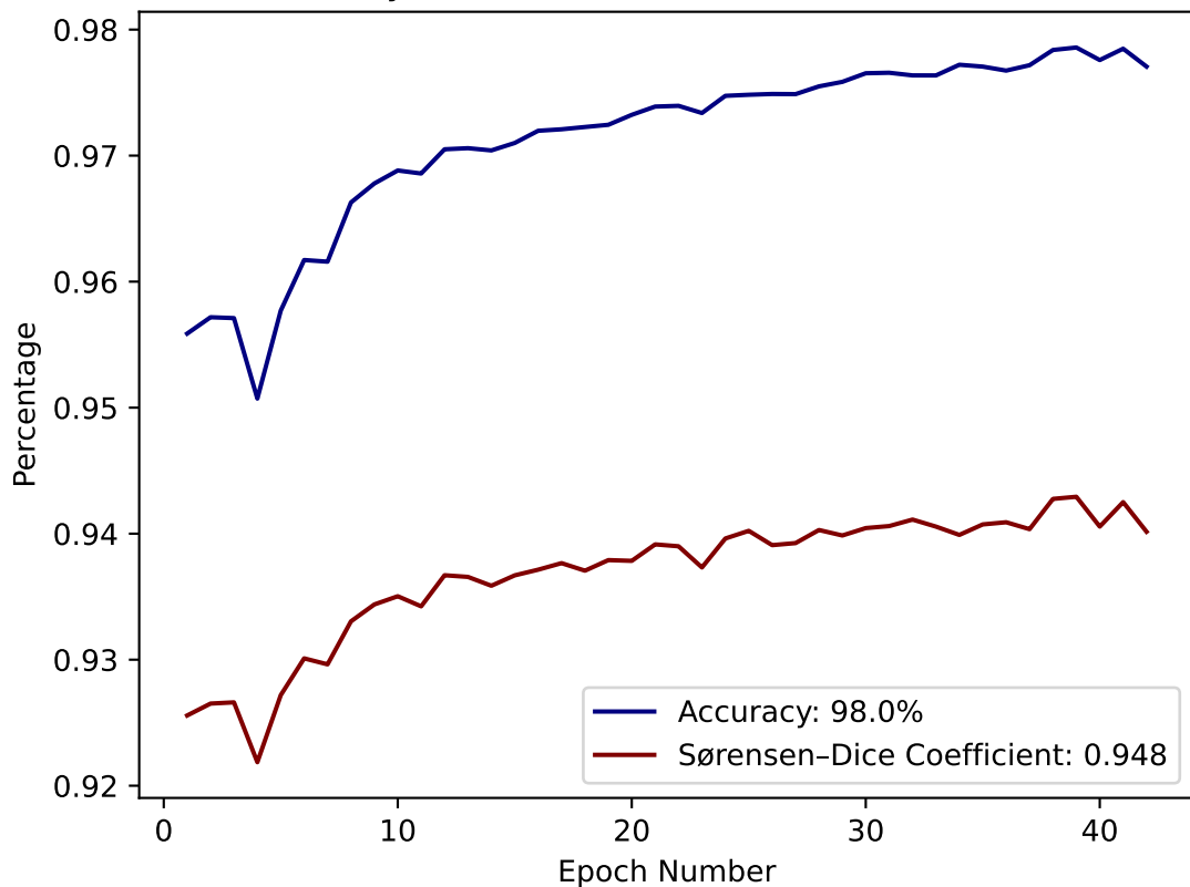
Multiclass Attention U-NET for Retinal Lesion Segmentation: Accuracy and Sørensen-Dice Coefficient Metrics
