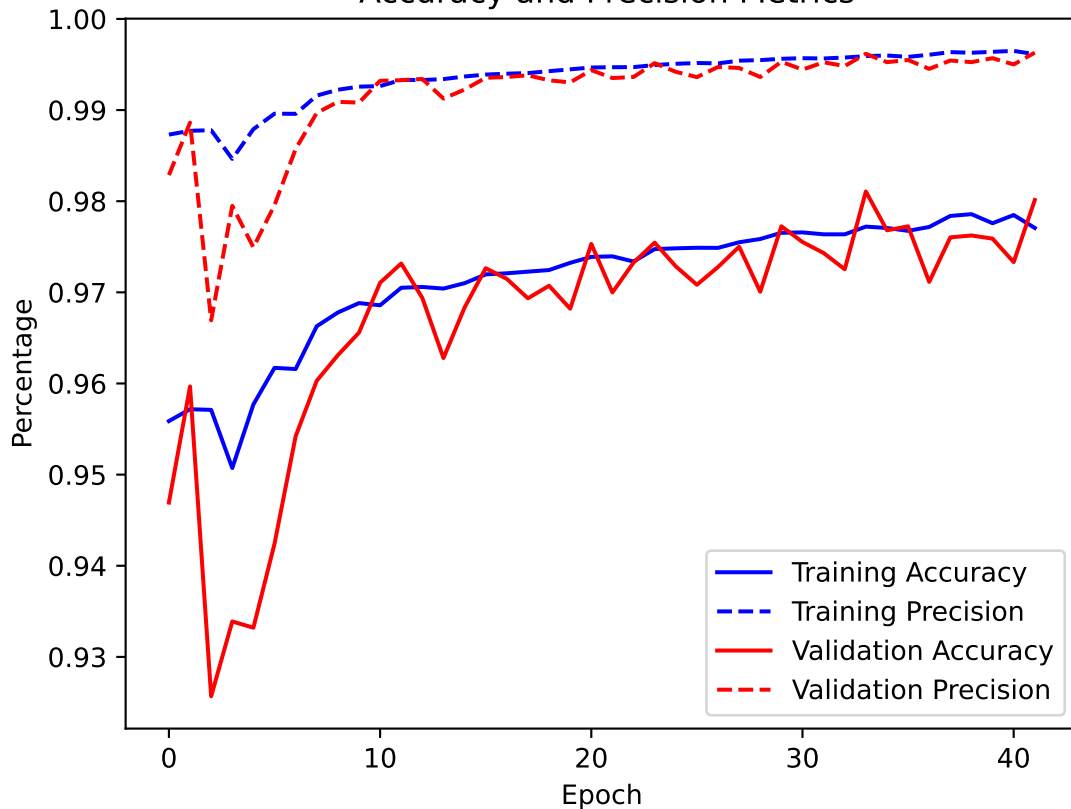
Multiclass Attention U-NET for Retinal Lesion Segmentation: Accuracy and Precision Metrics
