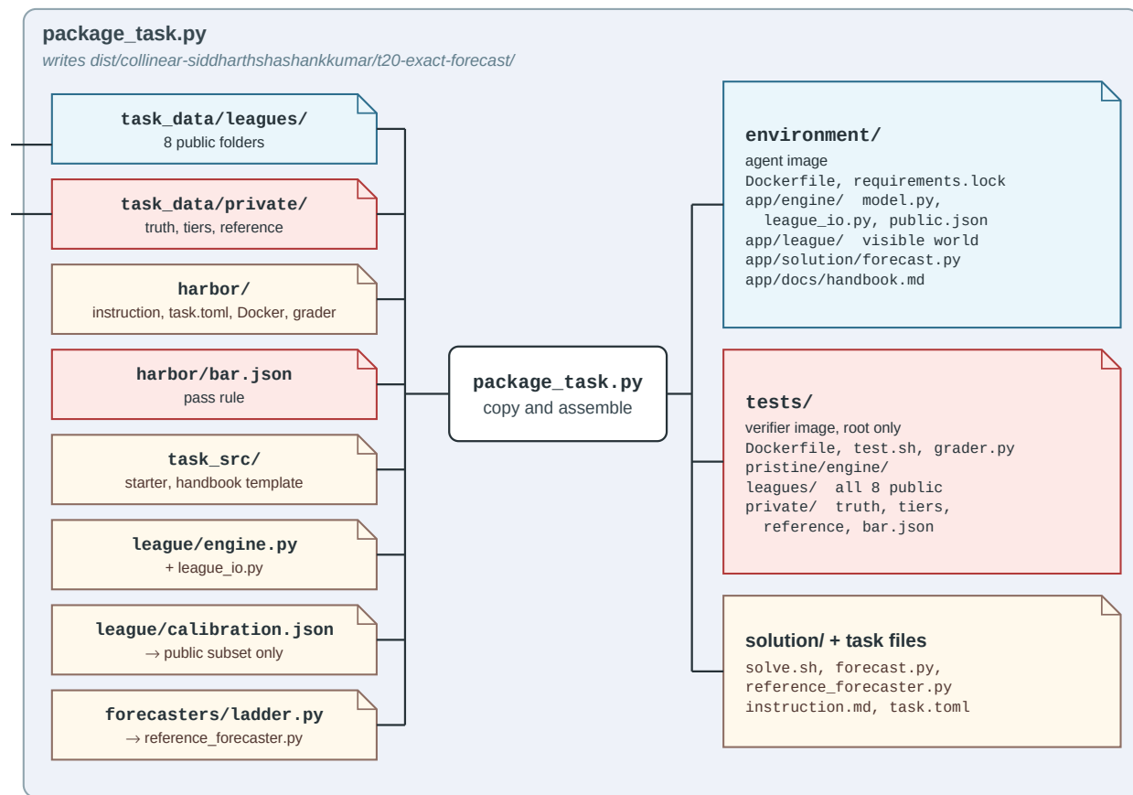
Figure 6: Building the eight worlds and packaging the task, continued. (b) package_task.py : the four source trees and the two sides of the task.
