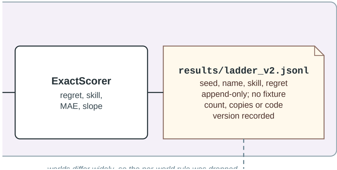
Figure 11: The experiments behind the bar, continued. (b) The ladder runner: scoring and the results log.
