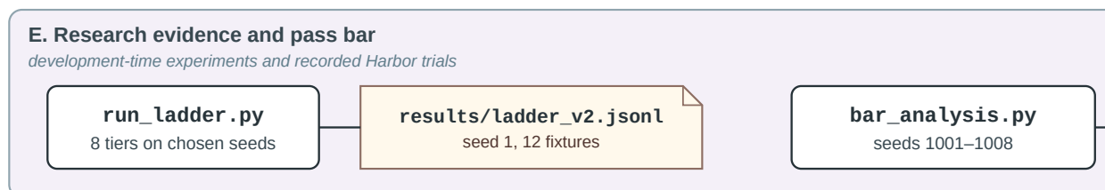
Figure 6: The whole system, as drawn from the repository, continued. (d) Research evidence and the pass bar, left half.
