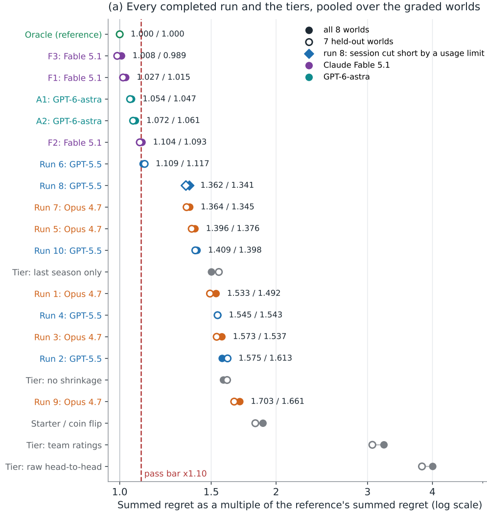
Figure 12: The ten pilots, world by world, and the ablations Left, every completed run of both generations and the ladder tiers as multiples of the reference's summed regret, on all eight worlds (filled) and the seven held out (hollow), against the 1.10 bar; run 8 is marked as the session cut short. Middle, every run world by world, with the values at or under the bar in bold. Right, the ablations of Section 6.3: each first-round program as submitted and after its one constant was changed, on held-out world c. Drawn from the job records, the build log and the ablation log by figures/src/pilot_results.py . (a) All ten runs and the ladder tiers, pooled over the graded worlds. Filled markers are all eight worlds, hollow the seven held out; run 8 is the session cut short by a usage limit.
