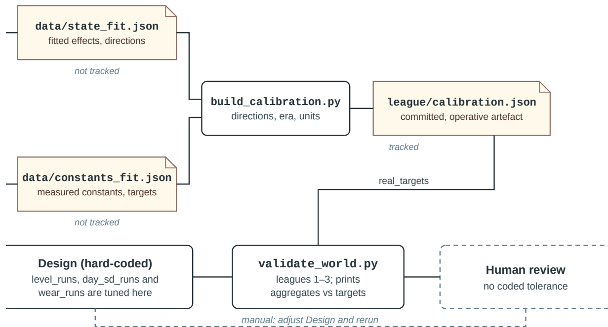
Figure 7: From the archive to the constants file, continued. (b) From the fitted files to the constants file, and the validation loop.
