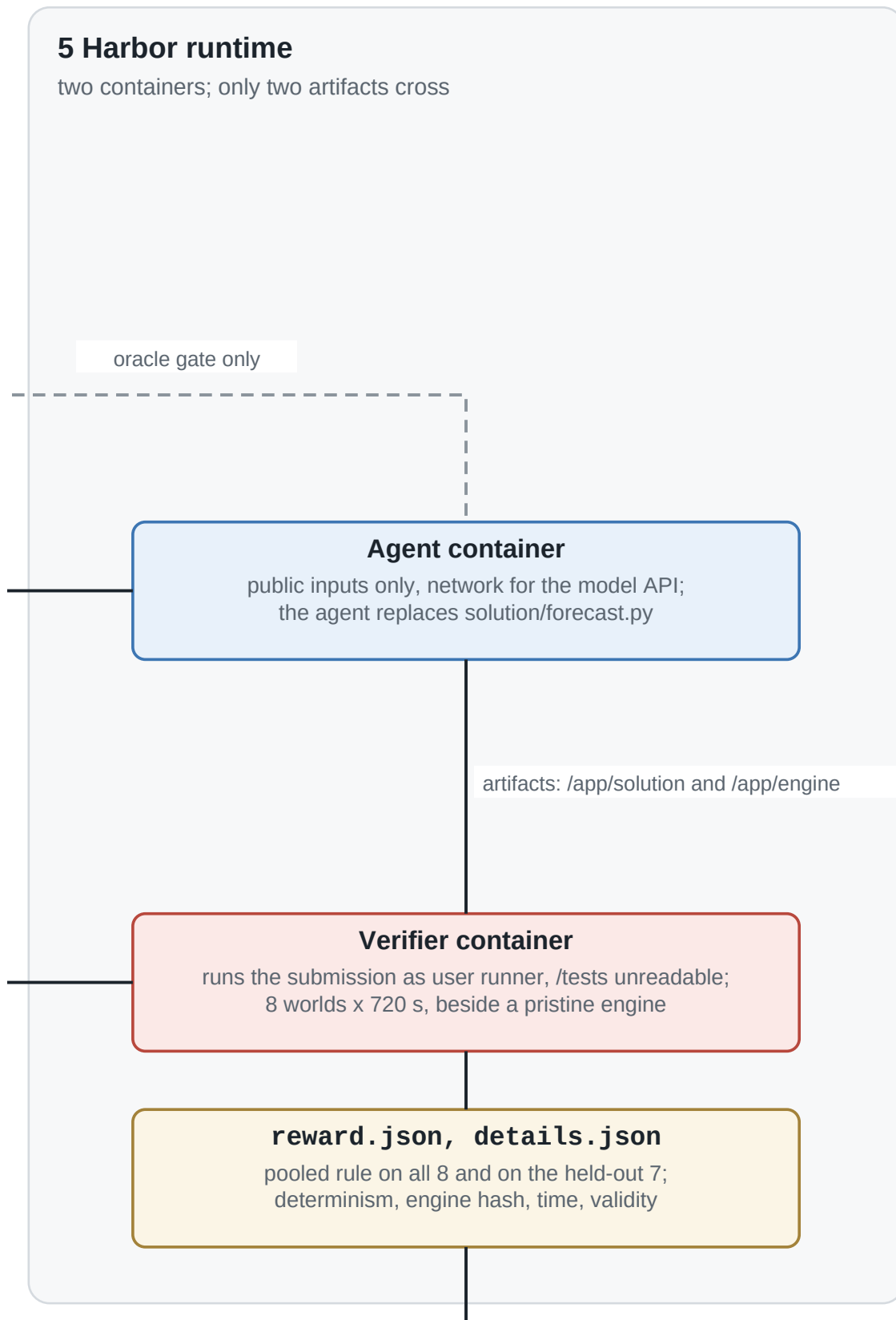
Figure 5: The project in six lanes, continued. (c) The Harbor runtime.
