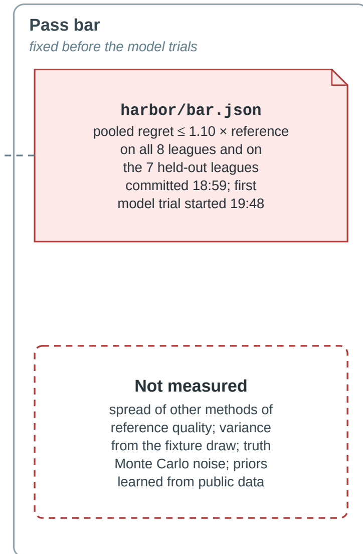
Figure 11: The experiments behind the bar, continued. (e) The pass bar as committed, and what was not measured.
