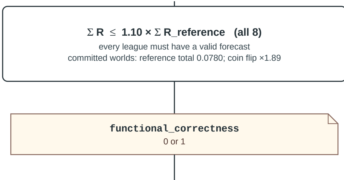
Figure 10: The pass rule and the reward composition, continued. (c) The rule on all eight worlds and the key it sets.
