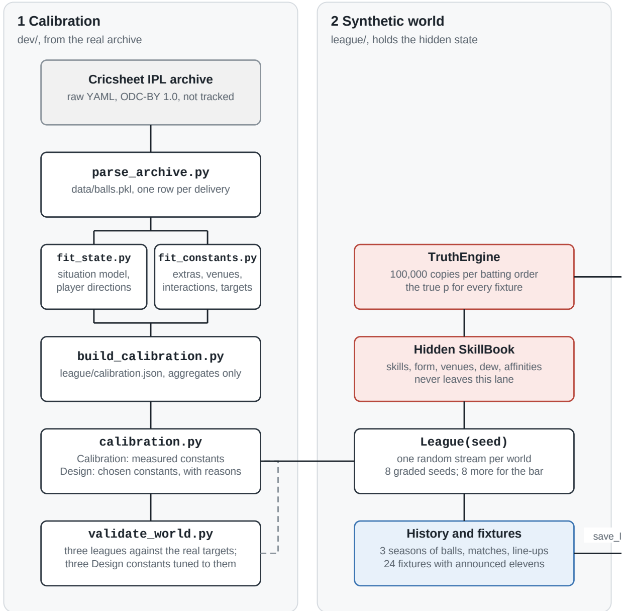
Figure 5: The project in six lanes Six lanes from the real archive to the documents. Blue nodes are what the agent sees, red what only the generator and the verifier hold. Every arrow is a data flow; the dashed ones are the oracle's install and the validation loop. (a) Calibration and the synthetic world.
