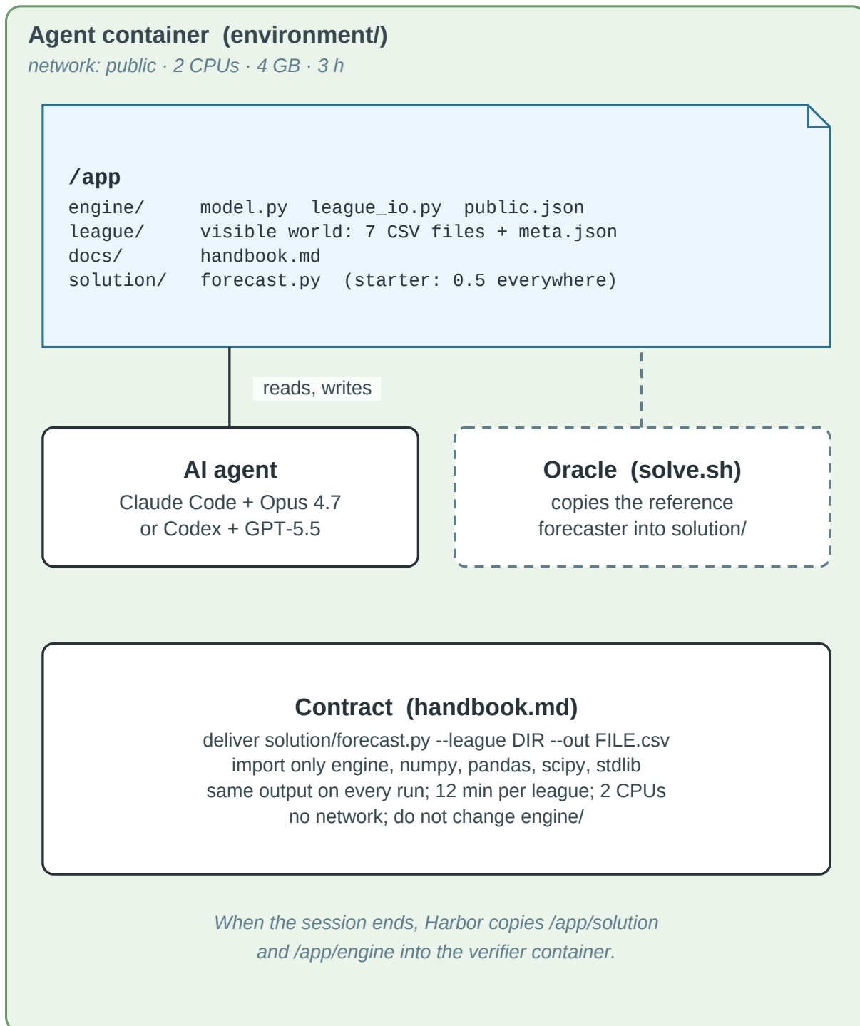
Figure 9: The two containers and the grader’s checks The agent sees only the public task. The verifier holds the answers, runs the submission as an unprivileged user beside a pristine engine, and applies the integrity, validity and scoring checks. (a) The agent container.
