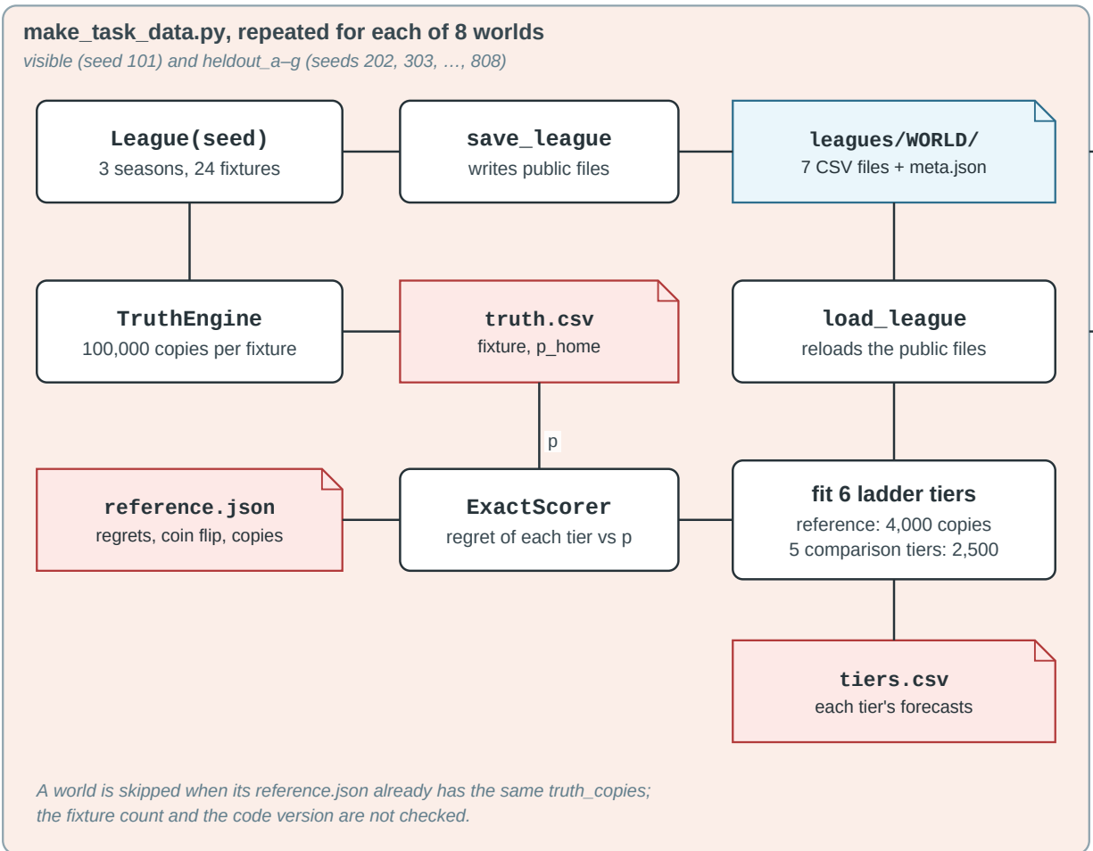
Figure 8: Building the eight worlds and packaging the task Left, what make_task_data.py does for each world, including the reload of the public files before the tiers are fitted. Right, the four source trees package_task.py assembles into the agent side, the verifier side and the oracle. (a) make_task_data.py , repeated for each of the eight worlds.
