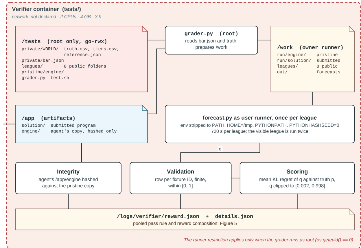
Figure 9: The two containers and the grader's checks, continued. (b) The verifier container and the grader's checks.
