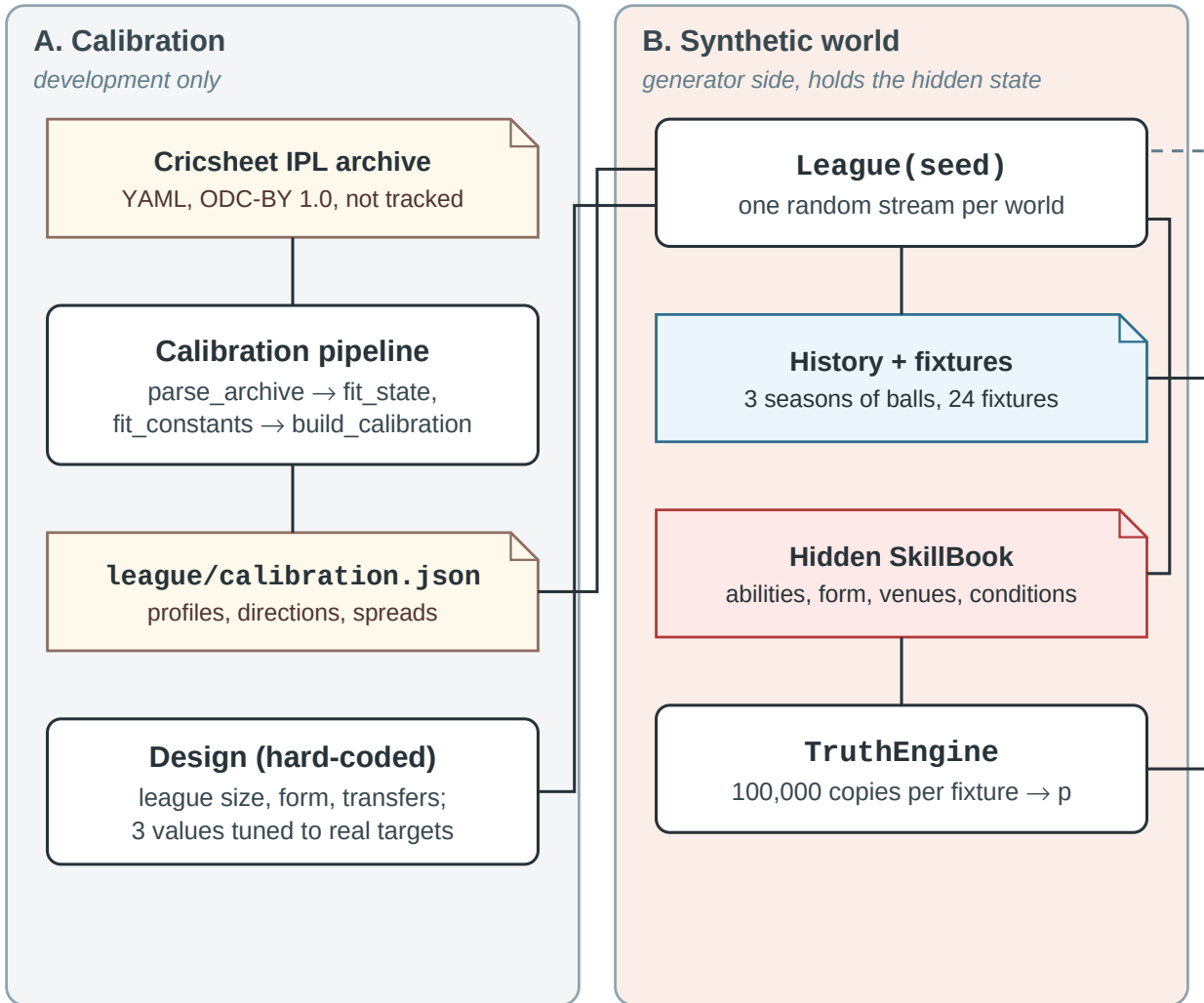
Figure 6: The whole system, as drawn from the repository Five zones: calibration from the real archive, the synthetic world that holds the hidden state, the task build and packaging, the Harbor runtime with its separate agent and verifier containers, and the research evidence behind the pass bar. (a) Calibration from the real archive, and the synthetic world that holds the hidden state.
