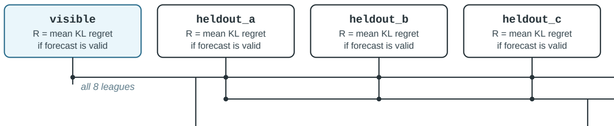
Figure 10: The pass rule and the reward composition One rule applied twice, to all eight worlds and to the seven held-out worlds, then the constraint and artifact checks, and how the four keys combine into the overall reward. (a) Each world's mean regret, left half.
