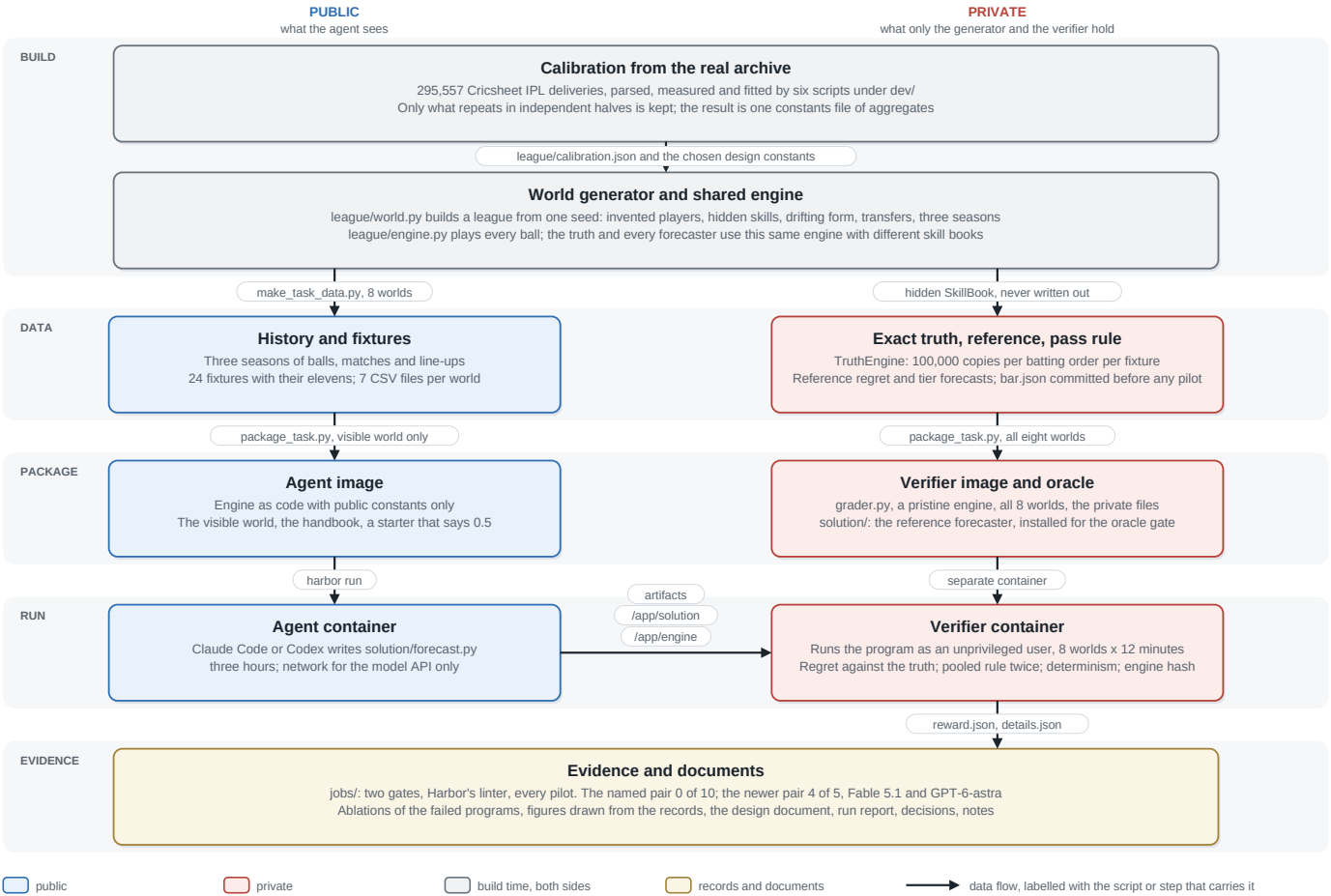
Figure 4: The system Two columns and five rows. The left column is what the agent sees, the right what only the generator and the verifier hold; the rows are build, data, package, run and evidence. Every arrow carries the name of the script or step that moves the data.
