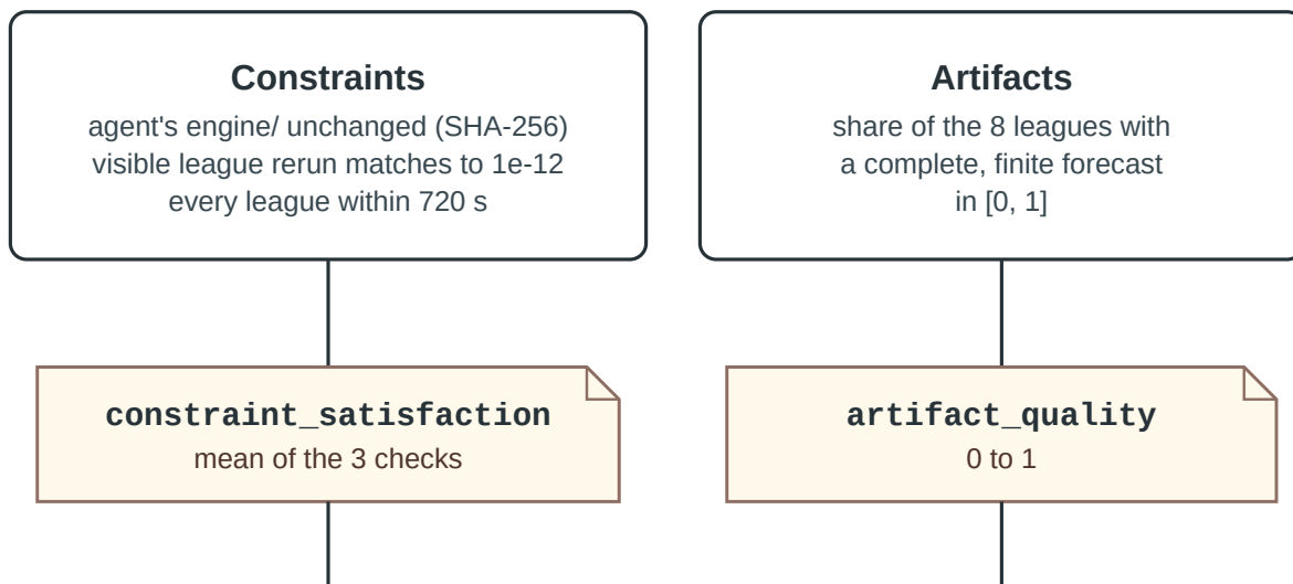
Figure 10: The pass rule and the reward composition, continued. (e) The constraint checks and the artifact check, and their keys.
