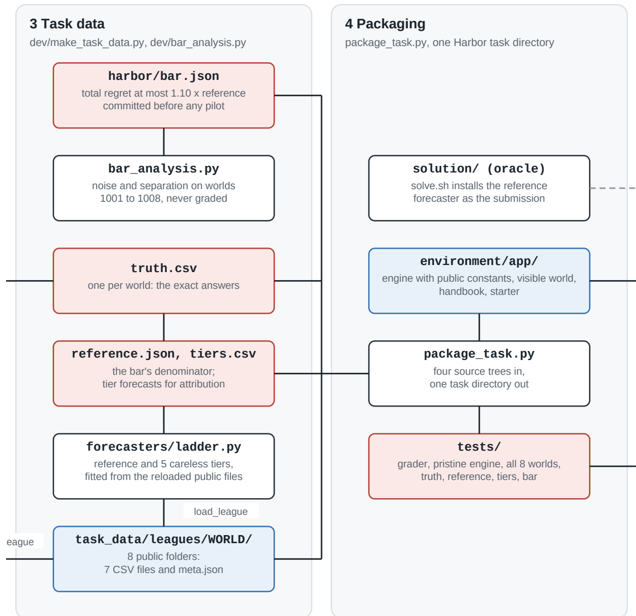
Figure 5: The project in six lanes, continued. (b) Task data and packaging.
