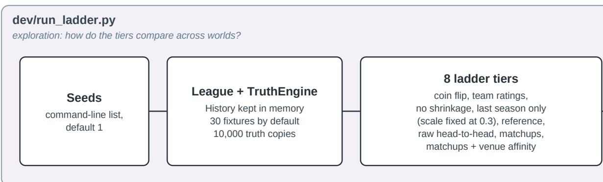
Figure 11: The experiments behind the bar The ladder runner across worlds, the bar analysis on eight worlds that are never graded, the quantities each measured, and the rule they produced. (a) The ladder runner: worlds, truth and the eight tiers.
