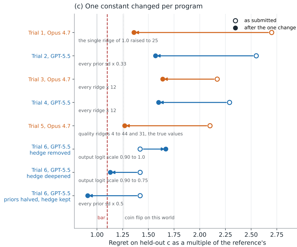
Figure 12: The ten pilots, world by world, and the ablations, continued. (c) The ablations of Section 6.3: each first-round program as submitted (hollow) and after its one constant was changed (filled), on held-out world c.
