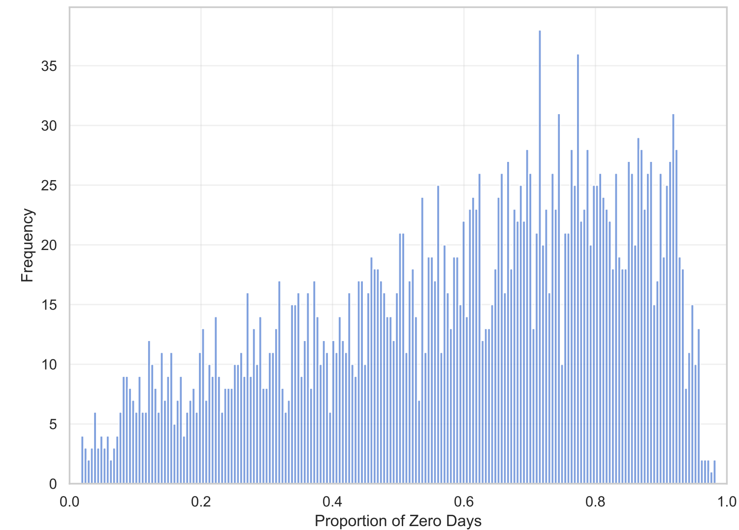
Zero Ratio
