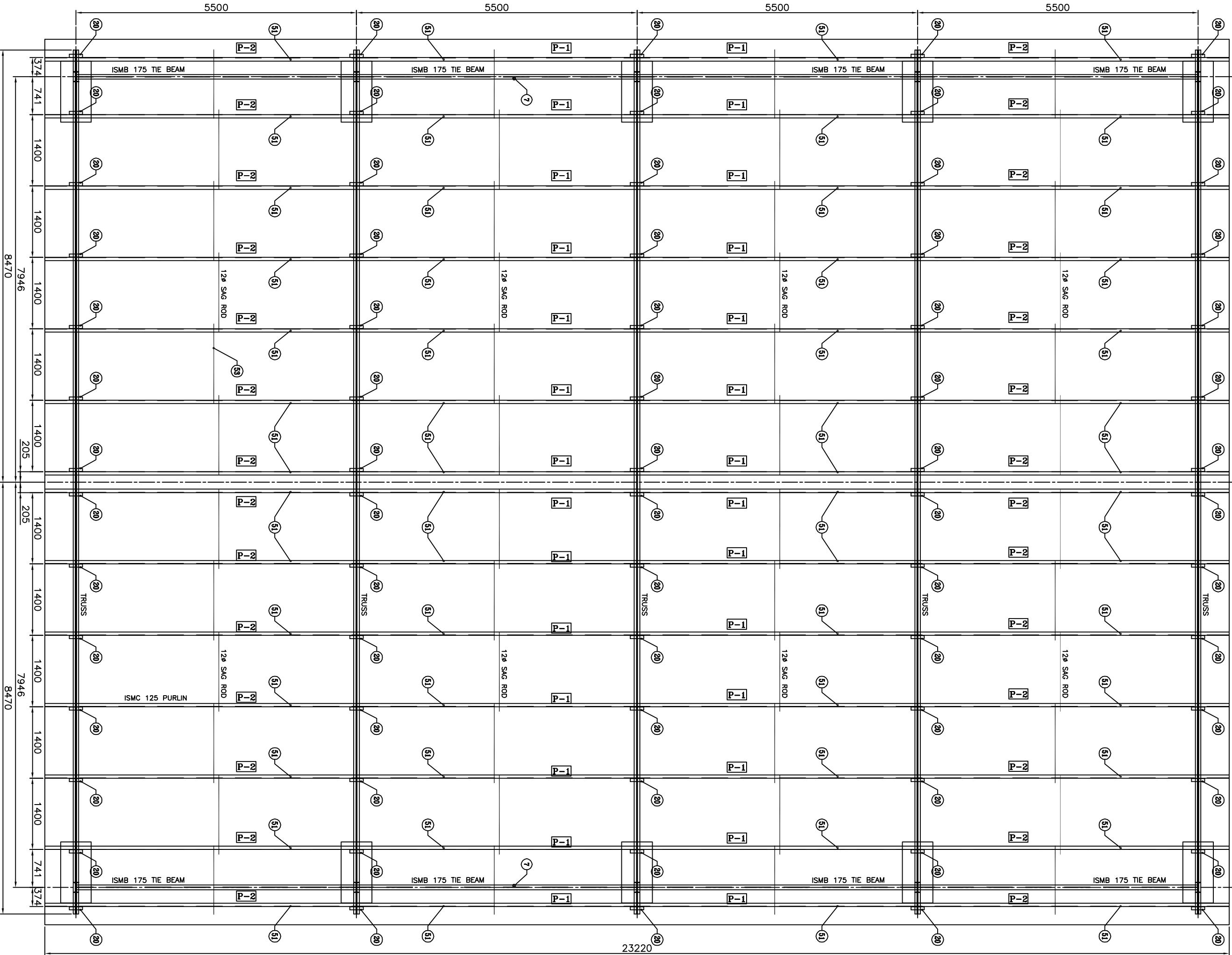
ROOF PLAN AT PURLING LEVEL
