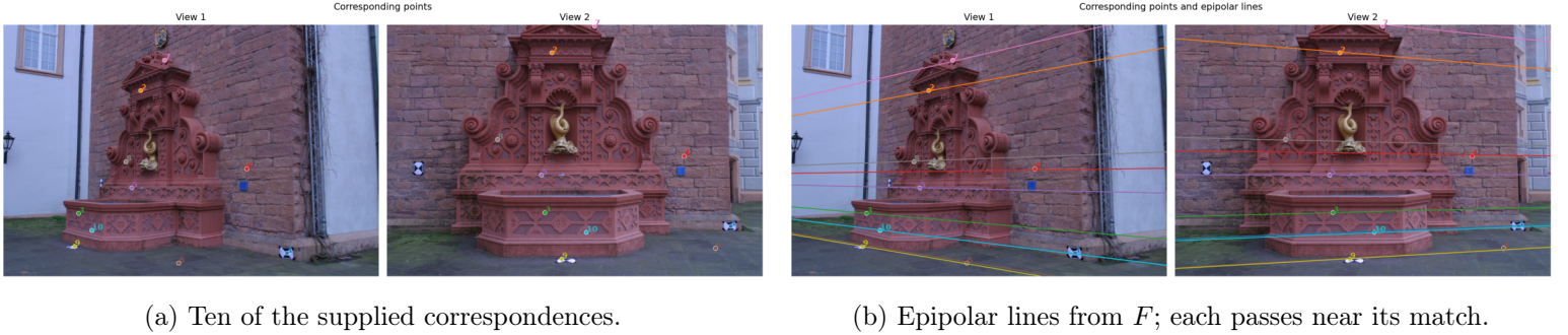
Figure 4: Two-view geometry on the fountain pair.
