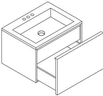
WALL-MOUNTED INTEGRATED BASIN* L60H40 DECK-MOUNTED TAPWARE (3 HOLES)
