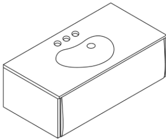
WALL-MOUNTED SMALL INTEGRATED BASIN* L60H30 DECK-MOUNTED TAPWARE (1 - 2 - 3 HOLES)
