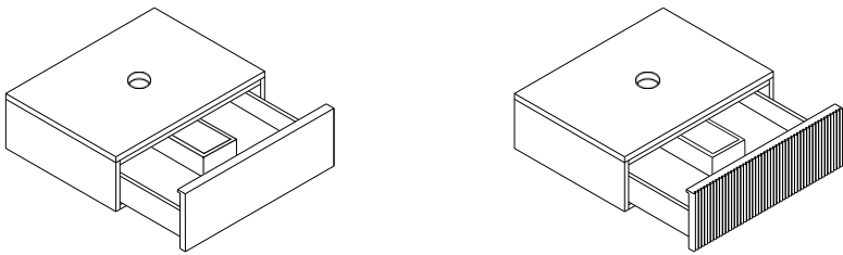
GENERIC COUNTERTOP MODULAR COMPONENT* L60H20 WALL-MOUNTED TAPWARE
