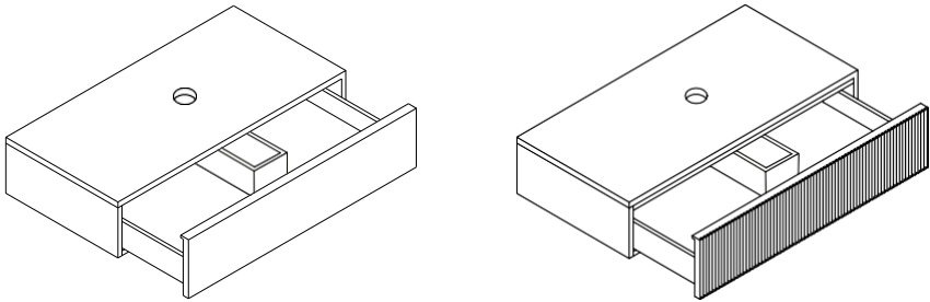
MODULO GENERICO PER COUNTERTOP BASIN* L90H20 WALL-MOUNTED TAPWARE
