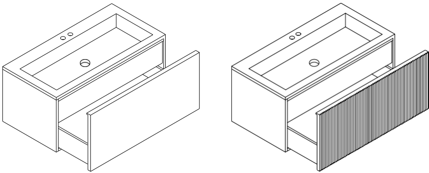
WALL-MOUNTED INTEGRATED BASIN* L90H40 DECK-MOUNTED TAPWARE (2 HOLES)
