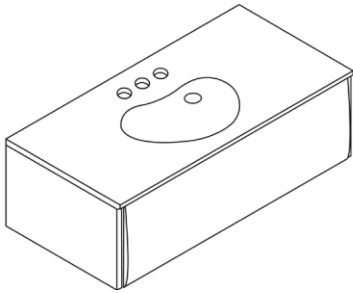
WALL-MOUNTED SMALL INTEGRATED BASIN* L70H30 DECK-MOUNTED TAPWARE (1 - 2 - 3 HOLES)
