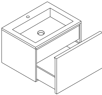
WALL-MOUNTED INTEGRATED BASIN* L60H40 DECK-MOUNTED TAPWARE (1 HOLE)
