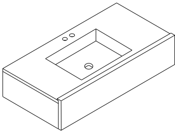
WALL-MOUNTED INTEGRATED BASIN* L90H20 DECK-MOUNTED TAPWARE (2 HOLES)
