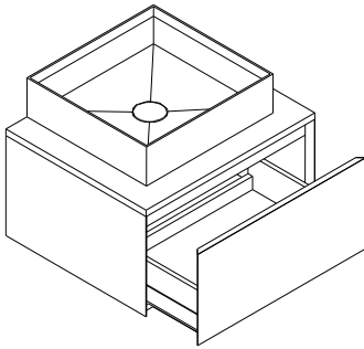
WALL-MOUNTED COUNTERTOP BASIN* L105H45 WALL-MOUNTED TAPWARE
