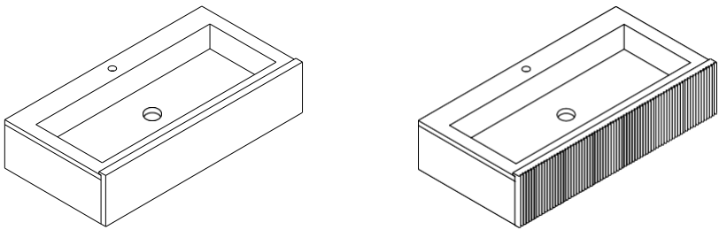
WALL-MOUNTED INTEGRATED BASIN* L90H20 DECK-MOUNTED TAPWARE (1 HOLE)
