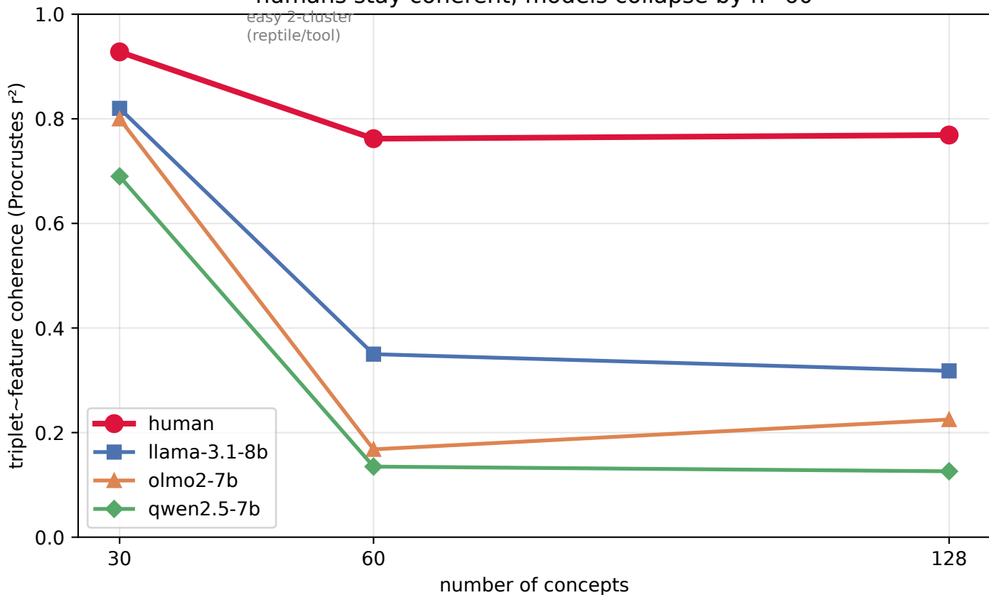
Coherence vs concept-set size: humans stay coherent, models collapse by n=60
