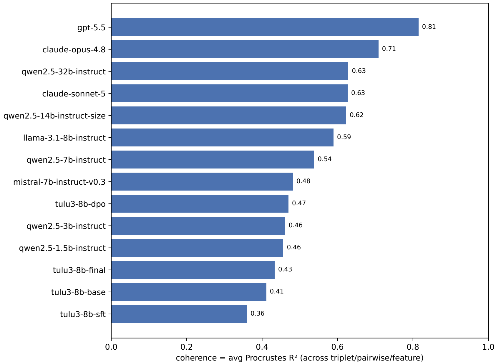
Semantic coherence (Procrustes R^2 )
