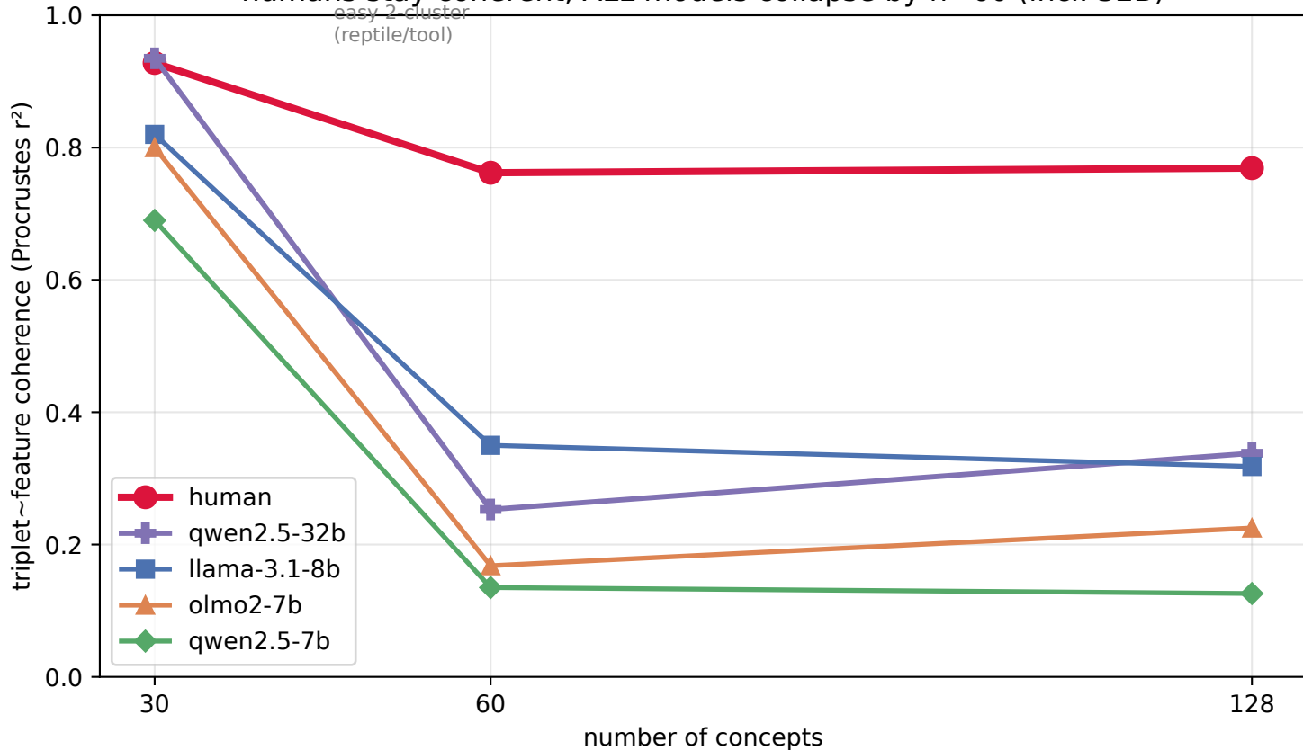
Coherence vs concept-set size: humans stay coherent, ALL models collapse by n=60 (incl. 32B)
