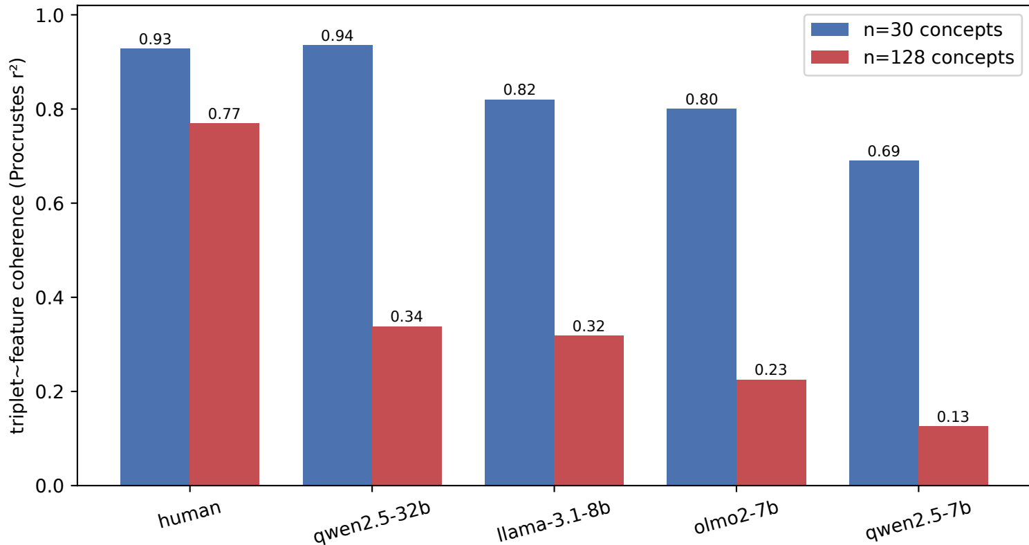
Conceptual coherence collapses with scale — for models, not humans
